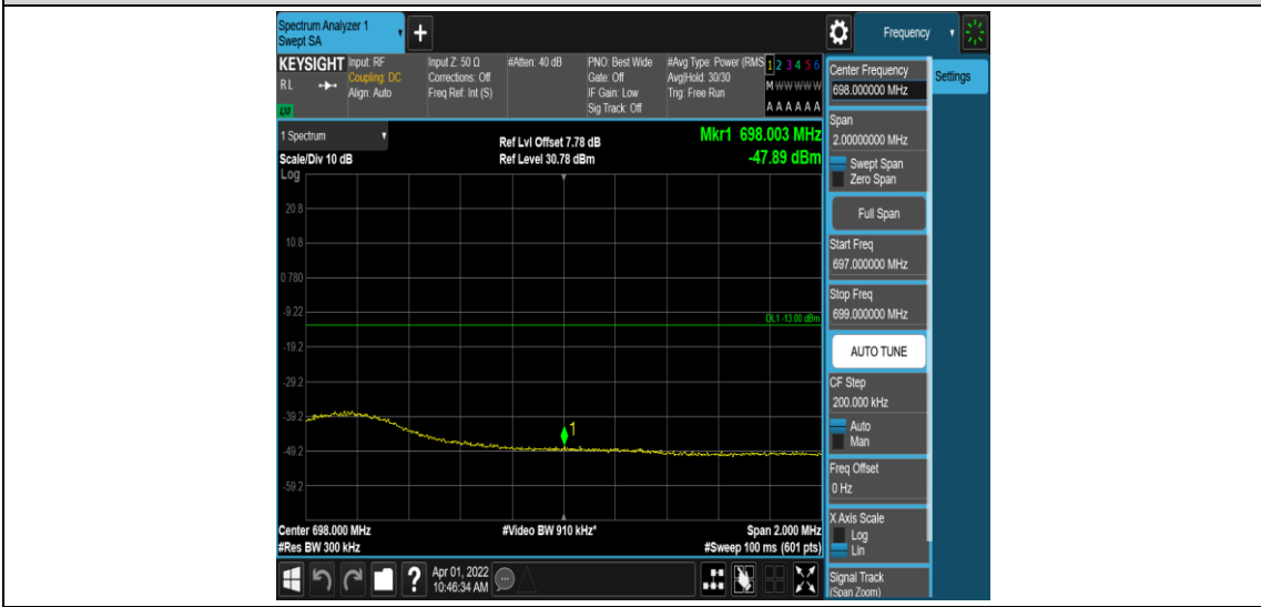
Band71-15MHz-16QAM-133397-1RB#0
