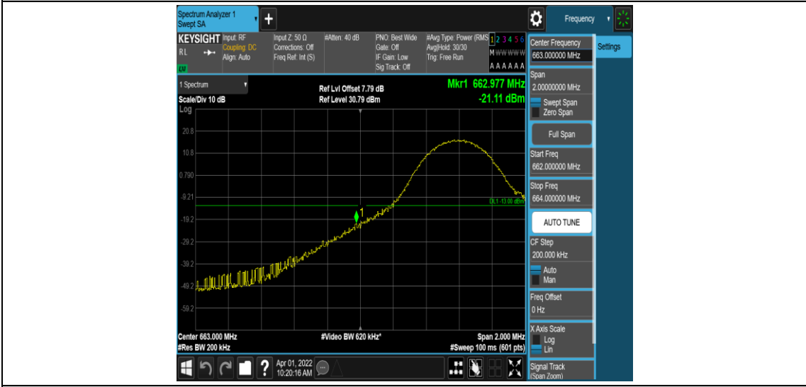
Band71-10MHz-16QAM-133172-1RB#0
