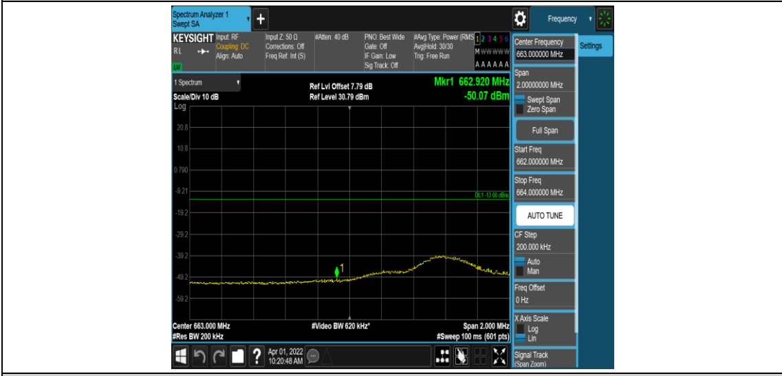
Band71-10MHz-16QAM-133172-1RB#49
