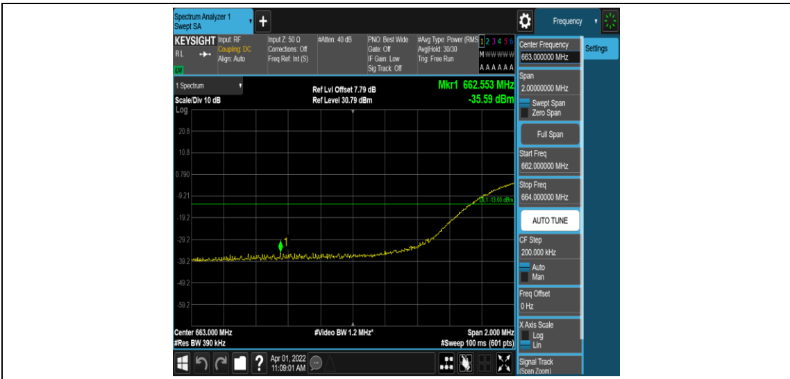
Band71-20MHz-16QAM-133222-100RB#0
