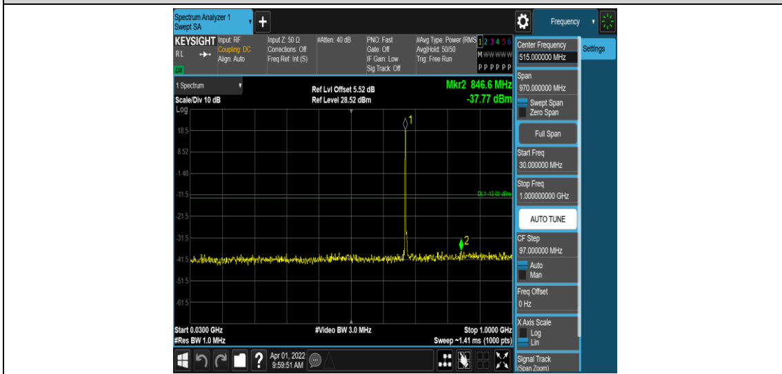
Band71-5MHz-QPSK-133297-1RB#0-Range3:30~1000MHz
