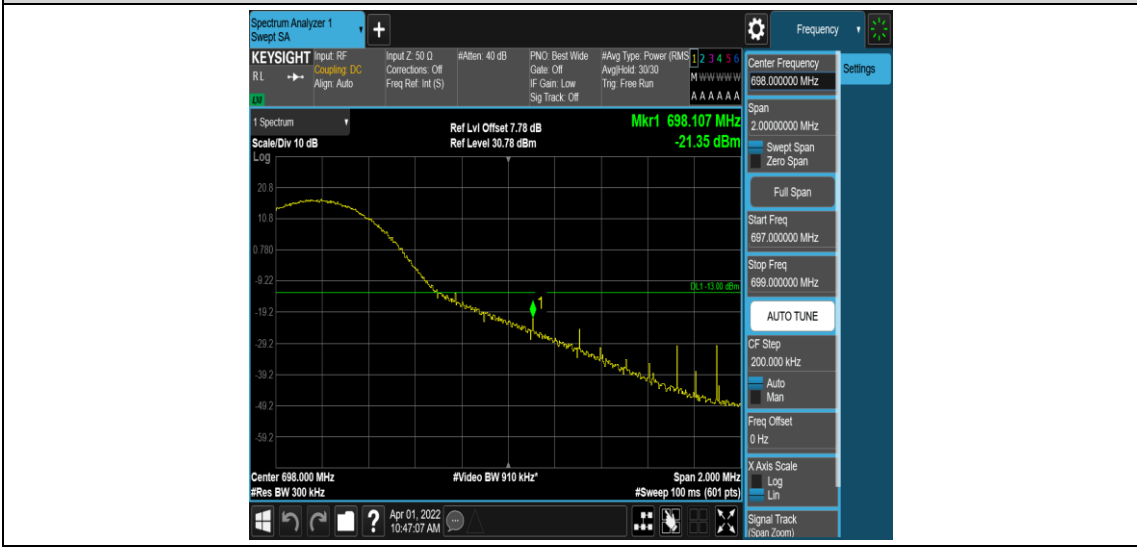
Band71-15MHz-16QAM-133397-1RB#74
