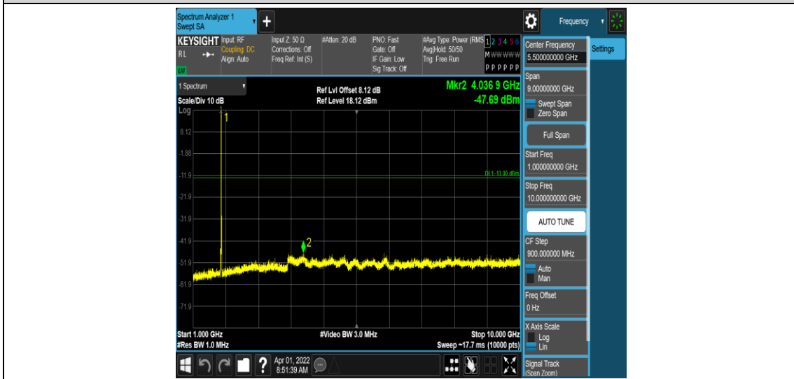
Band66-10MHz-QPSK-132622-1RB#0-Range4:1000~10000MHz
