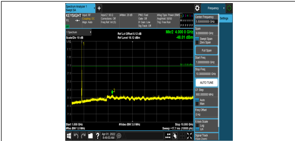
Band66-10MHz-QPSK-132322-1RB#0-Range4: 1000~10000MHz
