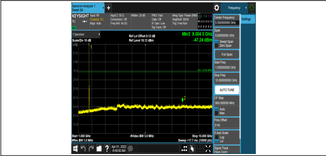
Band66-10MHz-16QAM-132022-1RB#0-Range4:1000~10000MHz
