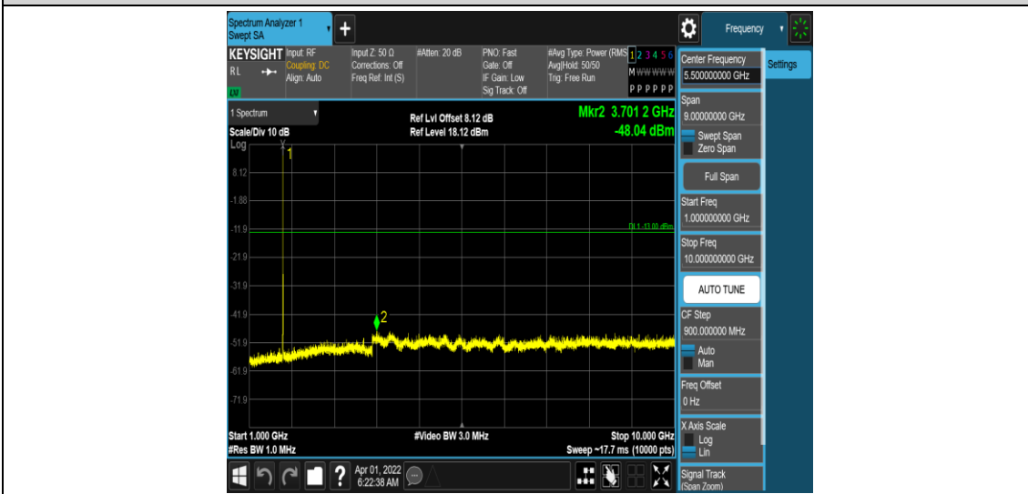
Band66-3MHz-16QAM-131987-1RB#0-Range4:1000~10000MHz
