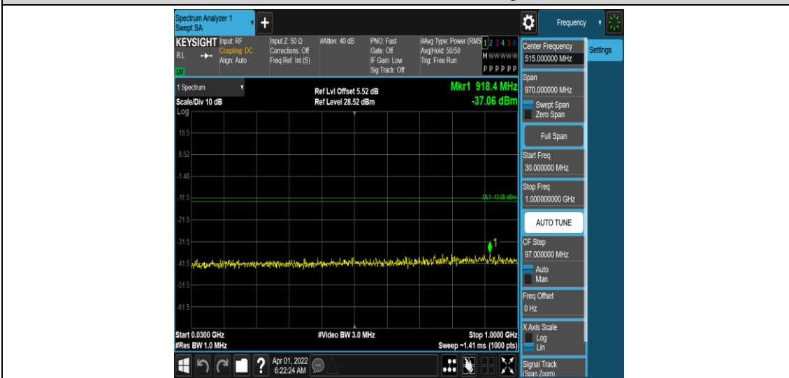
Band66-3MHz-16QAM-131987-1RB#0-Range3:30~1000MHz
