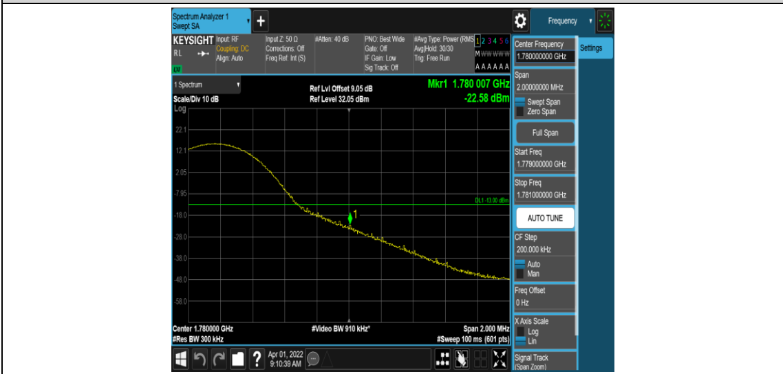
Band66-15MHz-QPSK-132597-1RB#74
