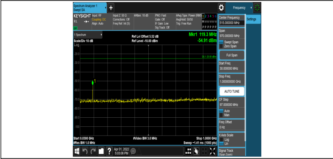
Band41-10MHz-16QAM-41540-1RB#0-Range3:30~1000MHz
