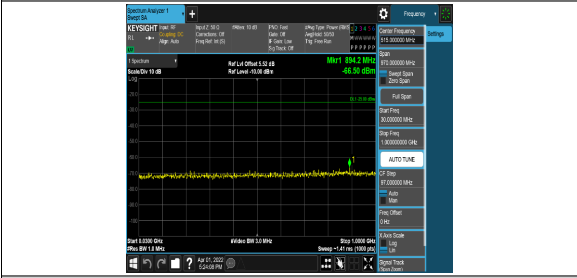
Band41-15MHz-QPSK-40620-1RB#0-Range3:30~1000MHz
