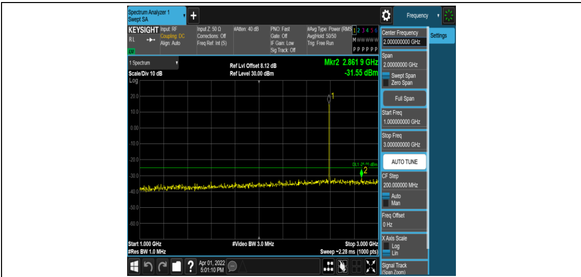
Band41-10MHz-16QAM-40620-1RB#0-Range4:1000~3000MHz
