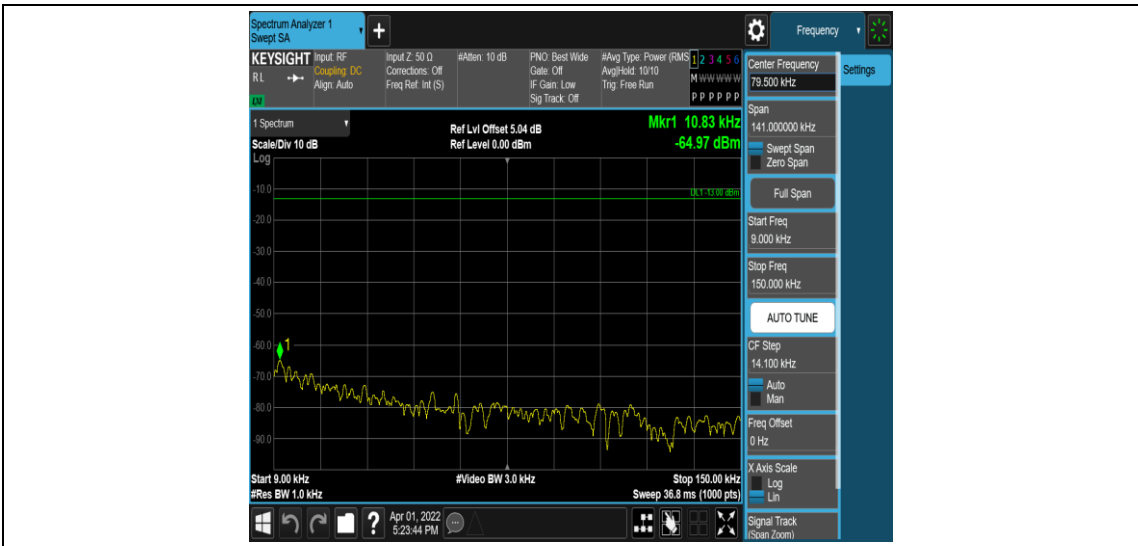
Band41-15MHz-QPSK-40620-1RB#0-Range1:0.009~0.15MHz
