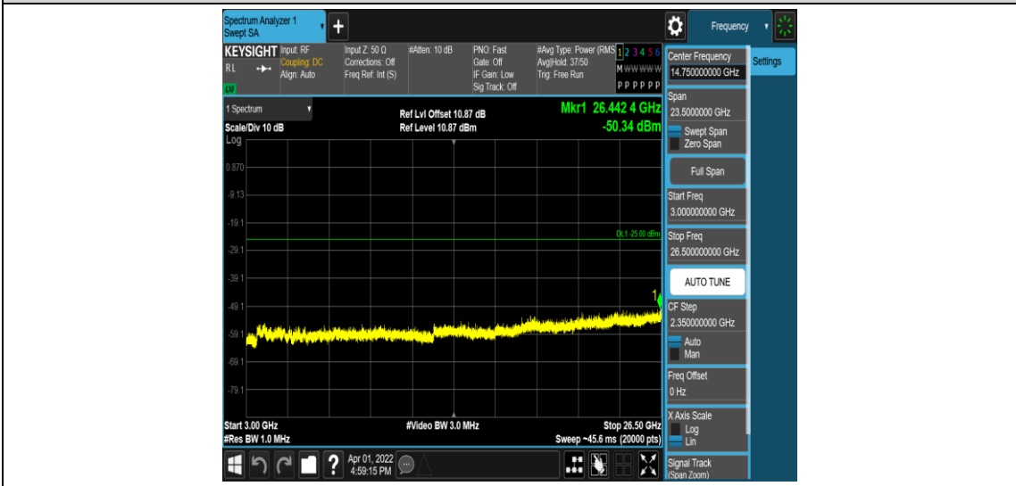
Band41-10MHz-16QAM-39700-1RB#0-Range5:3000~26500MHz
