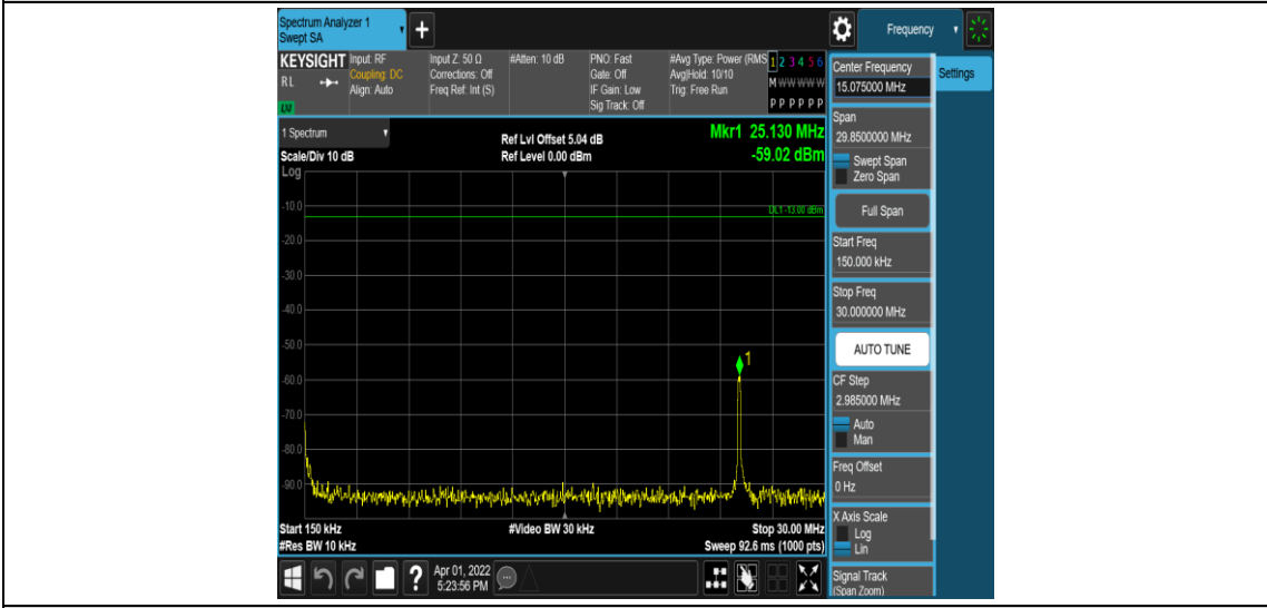
Band41-15MHz-QPSK-40620-1RB#0-Range2:0.15~30MHz
