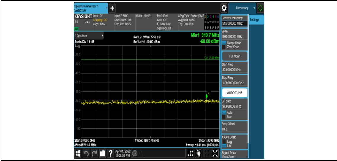
Band41-10MHz-16QAM-40620-1RB#0-Range3:30~1000MHz
