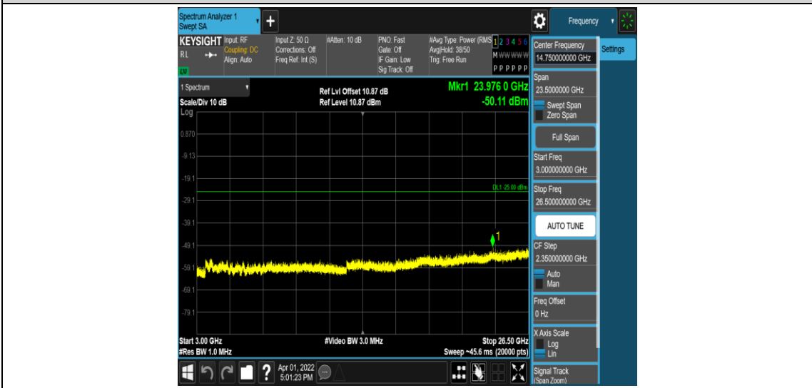
Band41-10MHz-16QAM-40620-1RB#0-Range5:3000~26500MHz
