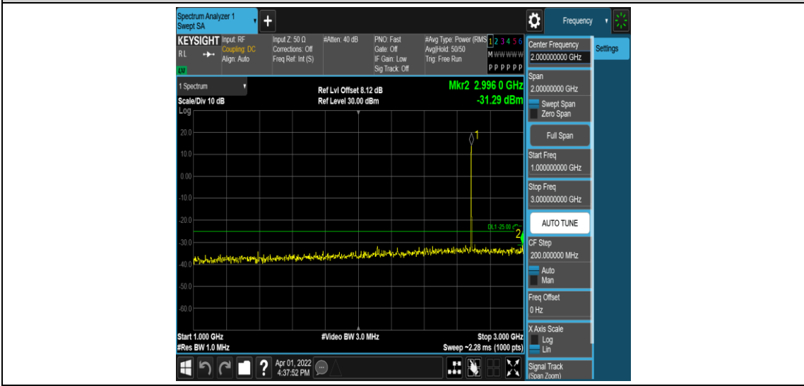
Band41-5MHz-16QAM-41565-1RB#0-Range4:1000~3000MHz
