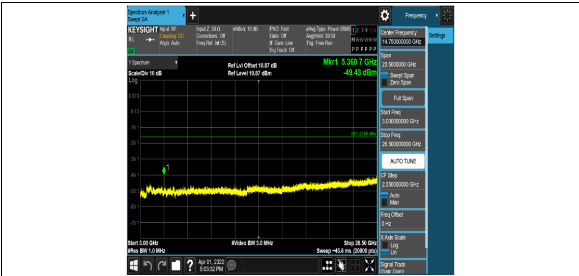
Band41-10MHz-16QAM-41540-1RB#0-Range5:3000~26500MHz
