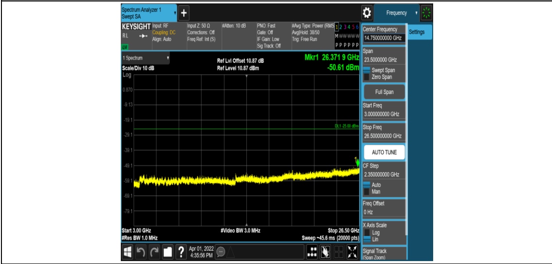
Band41-5MHz-16QAM-40620-1RB#0-Range5:3000~26500MHz
