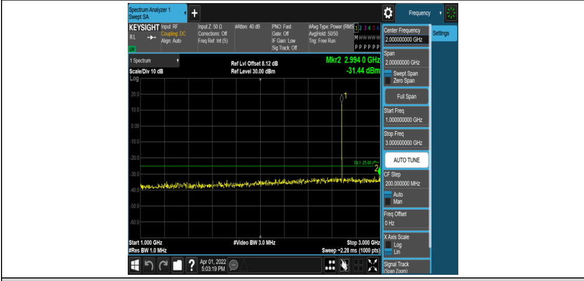
Band41-10MHz-16QAM-41540-1RB#0-Range4:1000~3000MHz
