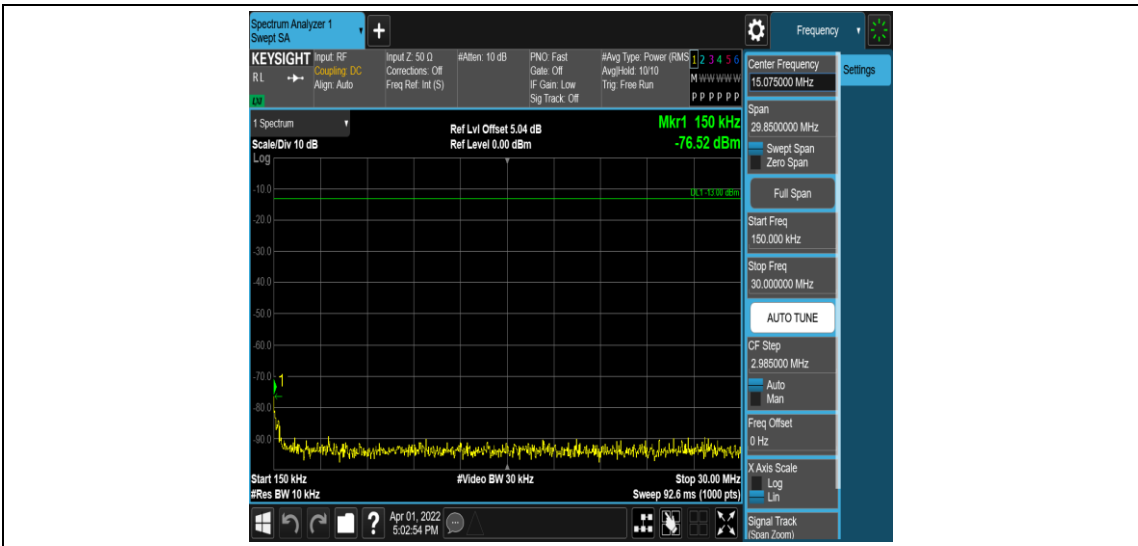
Band41-10MHz-16QAM-41540-1RB#0-Range2:0.15~30MHz
