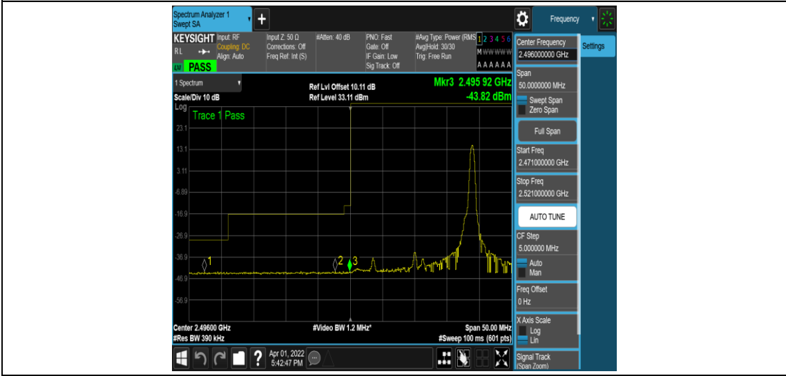
Band41-20MHz-QPSK-39750-1RB#99
