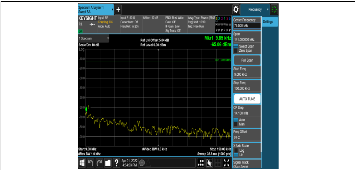
Band41-5MHz-QPSK-40620-1RB#0-Range1:0.009~0.15MHz
