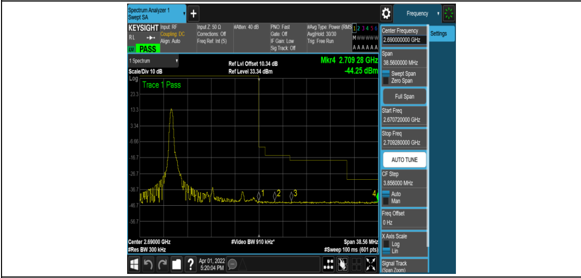
Band41-15MHz-16QAM-41515-1RB#0
