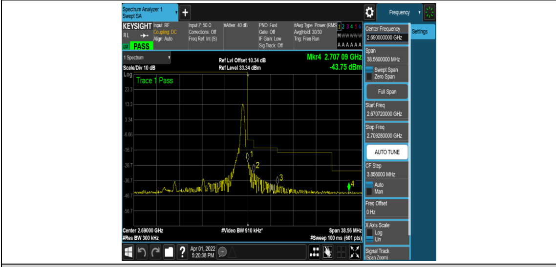
Band41-15MHz-16QAM-41515-1RB#74
