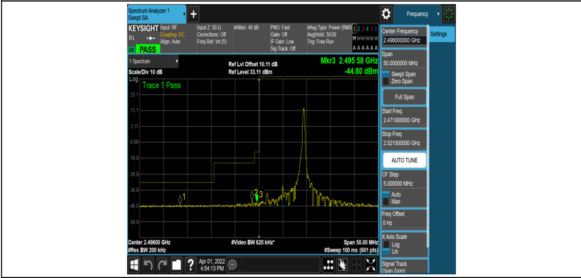
Band41-10MHz-QPSK-39700-1RB#49
