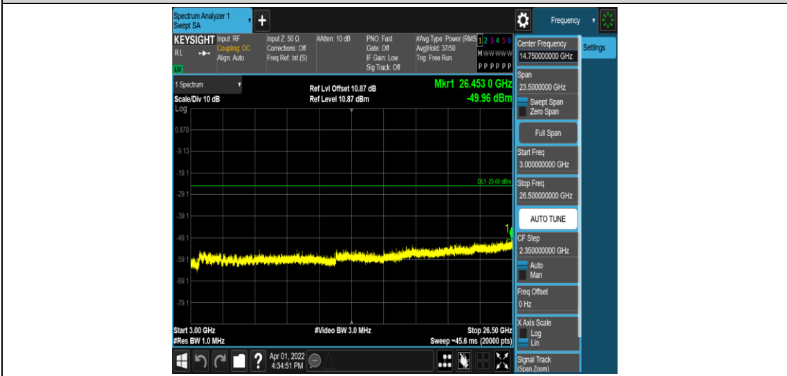
Band41-5MHz-QPSK-40620-1RB#0-Range5:3000~26500MHz
