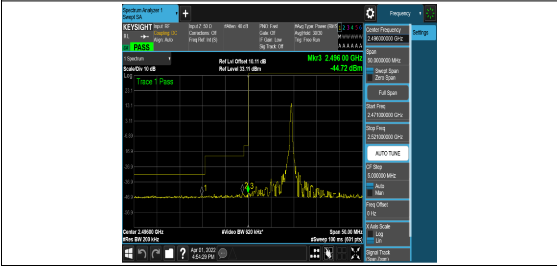
Band41-10MHz-16QAM-39700-1RB#49
