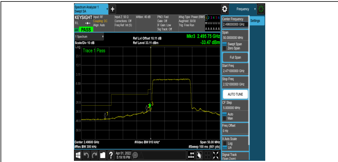
Band41-15MHz-16QAM-39725-75RB#0
