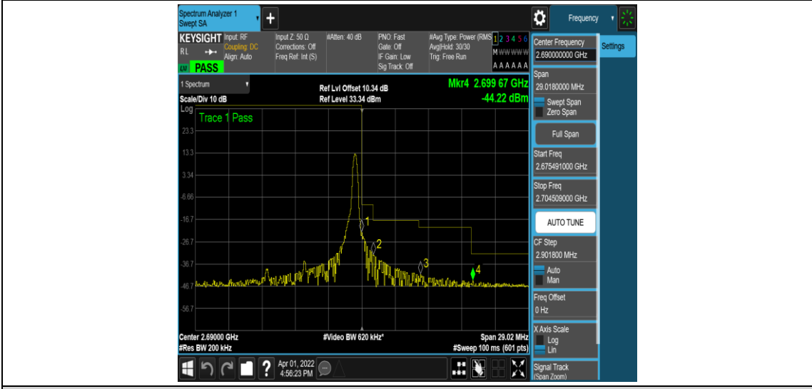
Band41-10MHz-16QAM-41540-1RB#49
