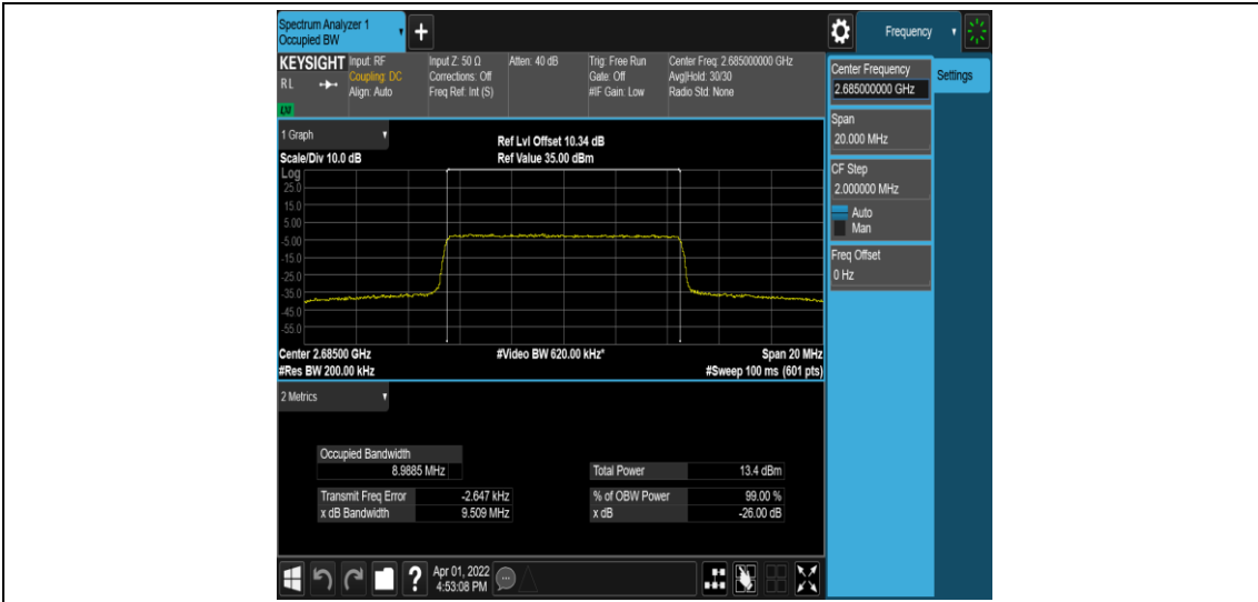
Band41-10MHz-16QAM-41540-50RB#0
