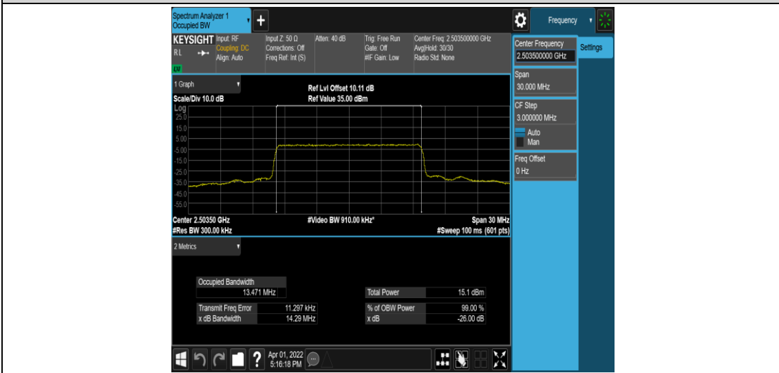
Band41-15MHz-QPSK-39725-75RB#0
