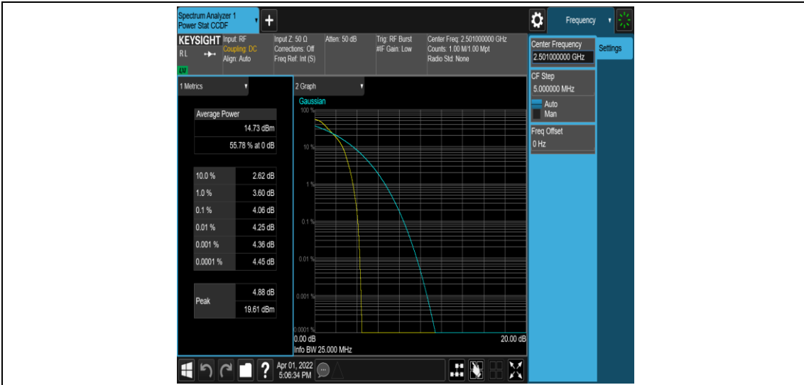
Band41-10MHz-QPSK-39700-1RB#0
