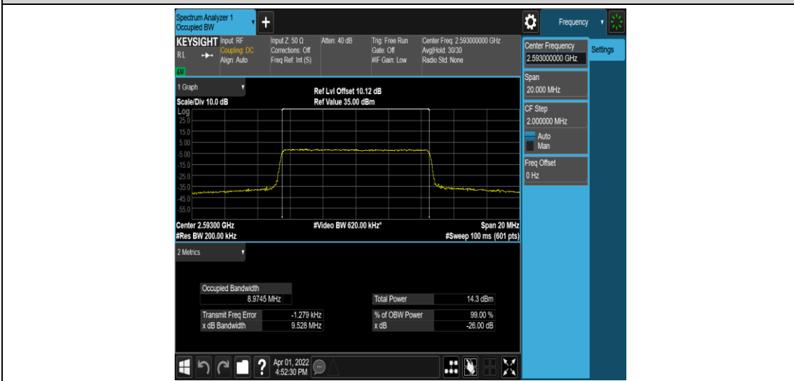
Band41-10MHz-QPSK-40620-50RB#0
