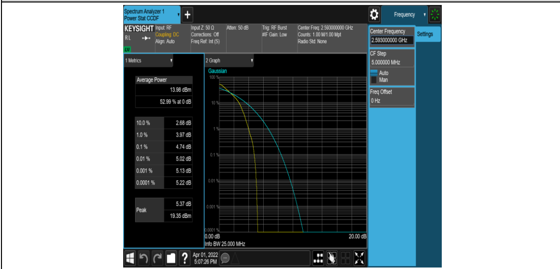
Band41-10MHz-QPSK-40620-1RB#0
