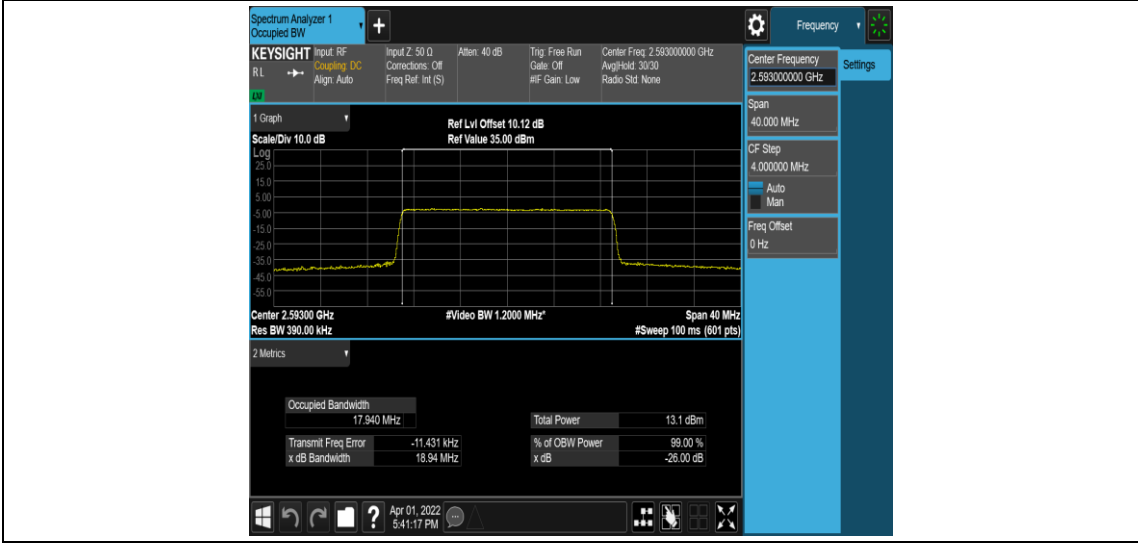
Band41-20MHz-16QAM-40620-100RB#0
