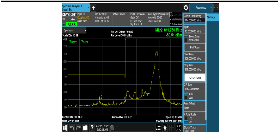
Band26-3MHz-16QAM-26705-1RB#14
