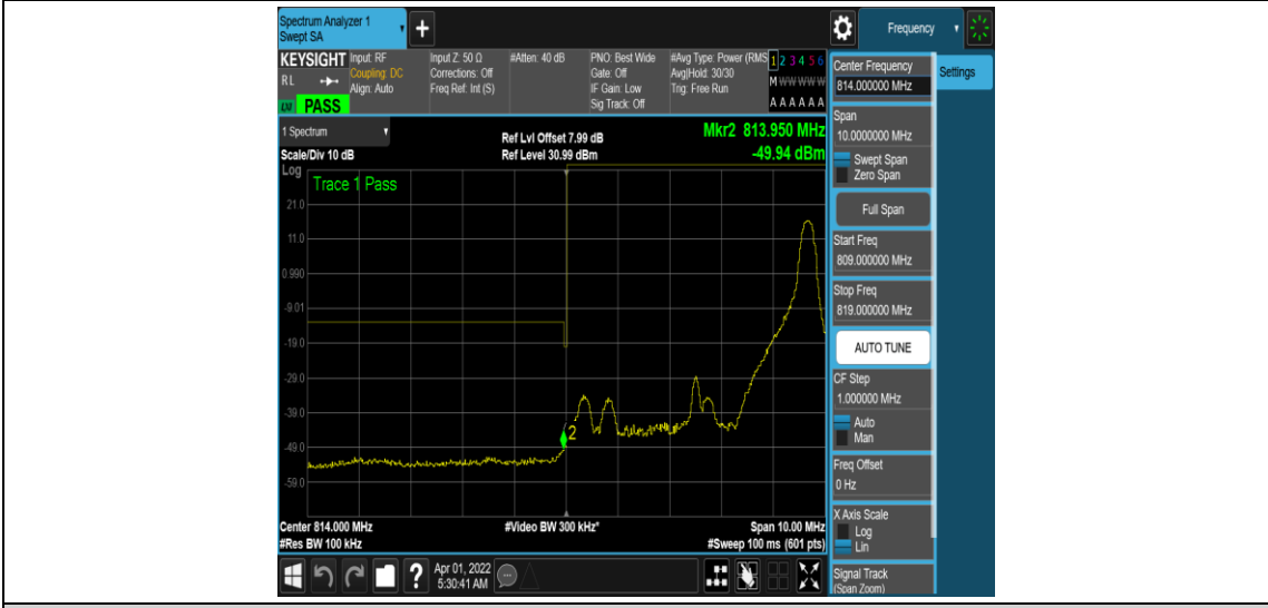
Band26-5MHz-QPSK-26715-1RB#24
