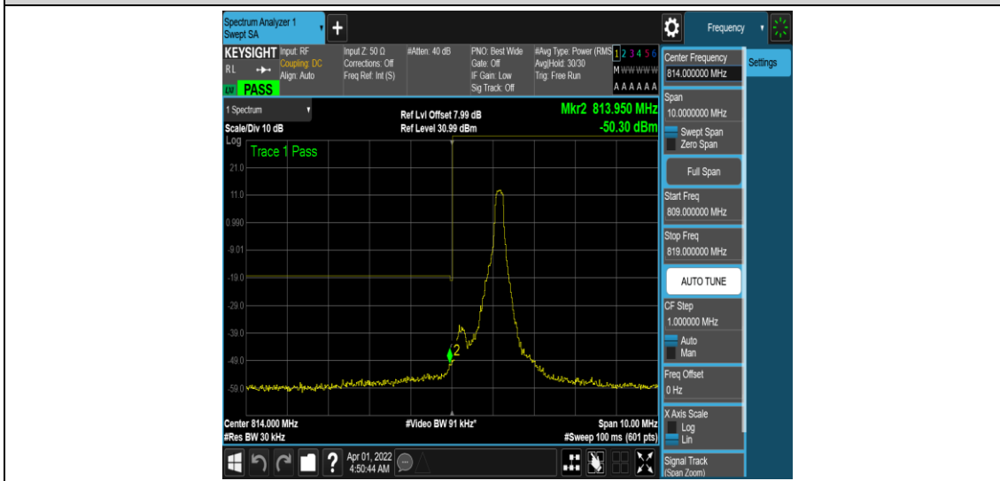
Band26-1.4MHz-QPSK-26697-1RB#5
