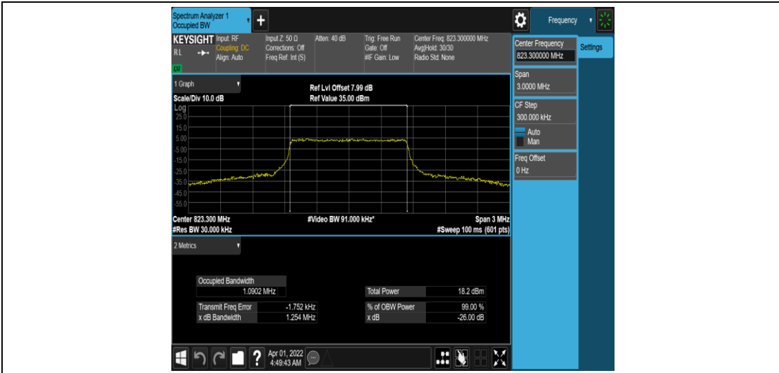
Band26-1.4MHz-16QAM-26783-6RB#0
