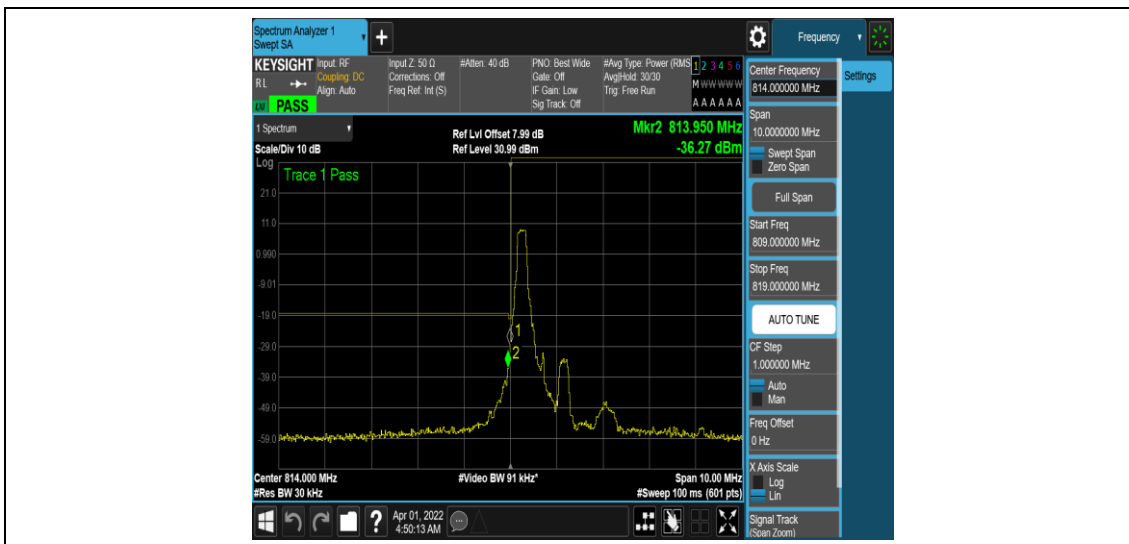
Band26-1.4MHz-QPSK-26697-1RB#0
