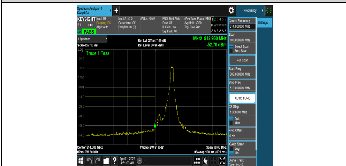
Band26-1.4MHz-16QAM-26697-1RB#5
