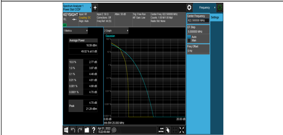
Band26-3MHz-16QAM-26775-1RB#0
