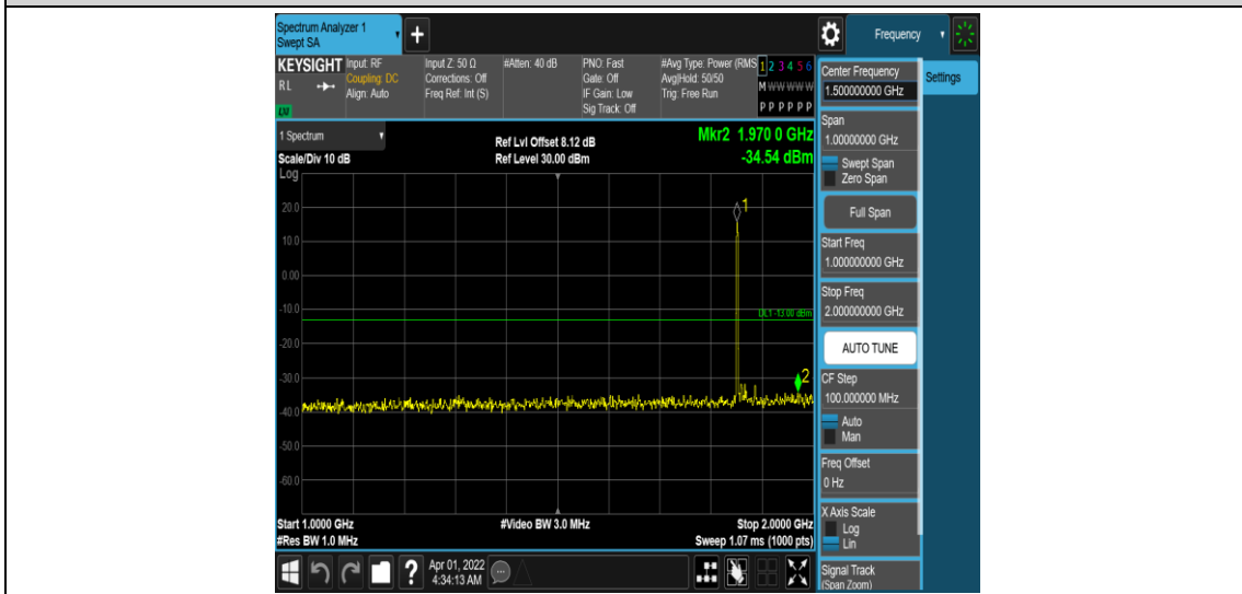
Band25-20MHz-16QAM-26140-1RB#0-Range4:1000~2000MHz
