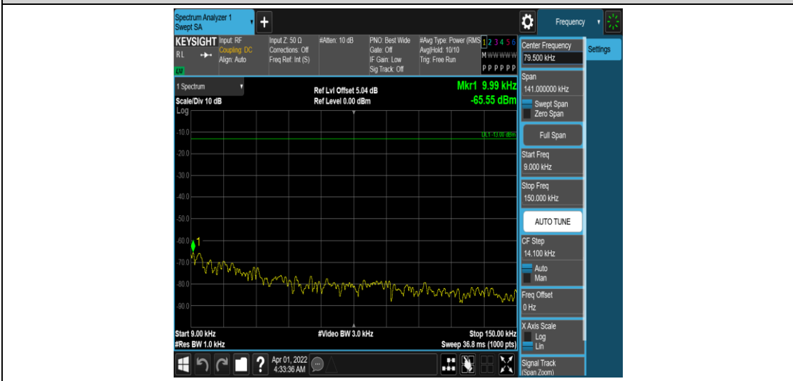
Band25-20MHz-16QAM-26140-1RB#0-Range1:0.009~0.15MHz
