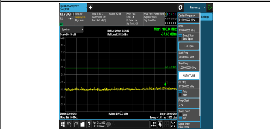
Band25-15MHz-16QAM-26615-1RB#0-Range3:30~1000MHz
