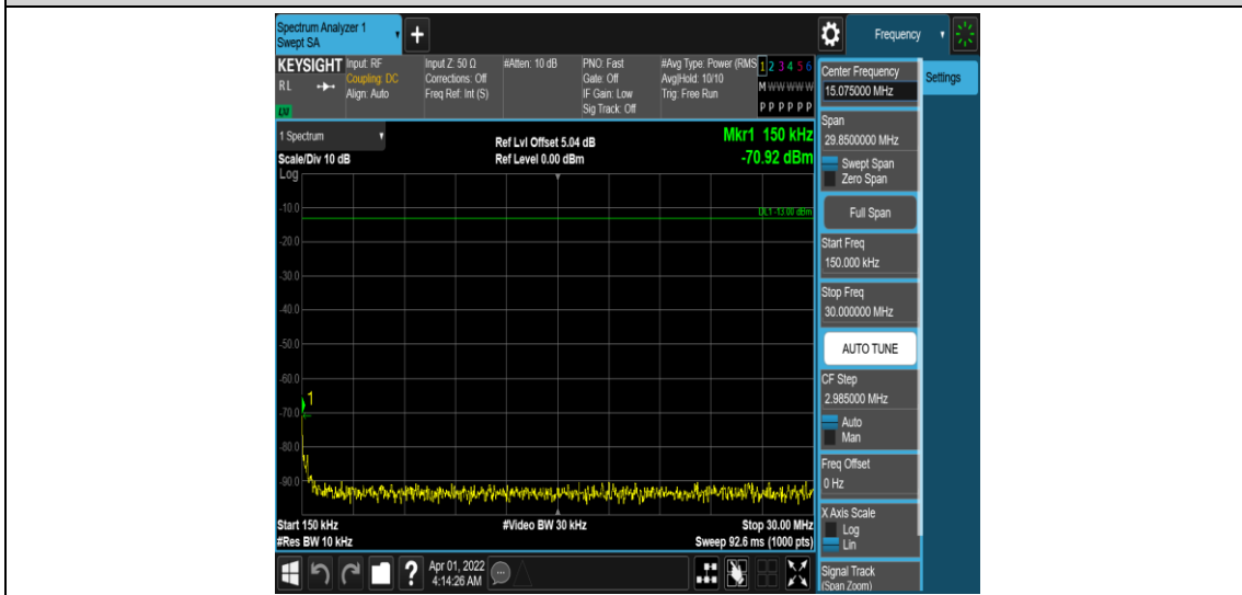
Band25-15MHz-16QAM-26365-1RB#0-Range2:0.15~30MHz
