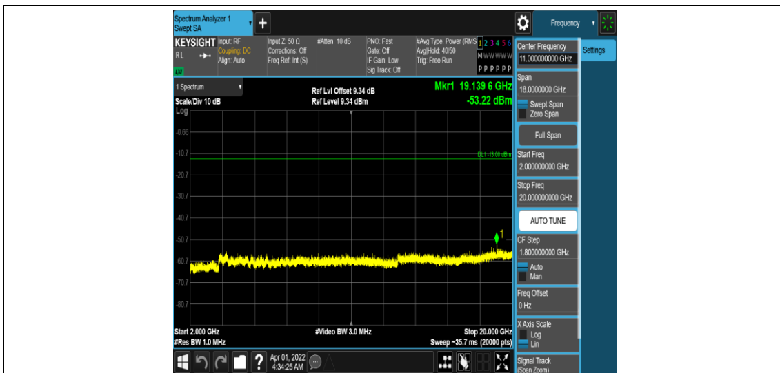
Band25-20MHz-16QAM-26140-1RB#0-Range5:2000~20000MHz
