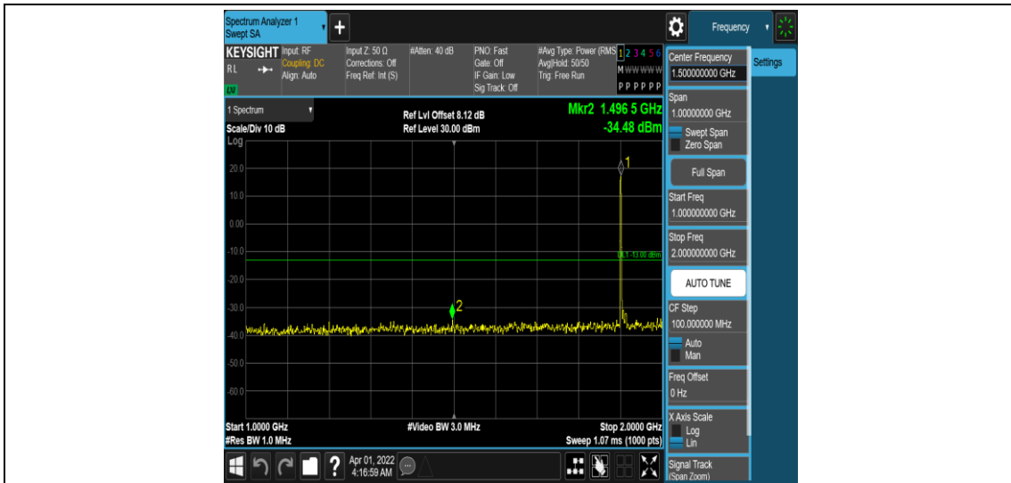
Band25-15MHz-16QAM-26615-1RB#0-Range4:1000~2000MHz
