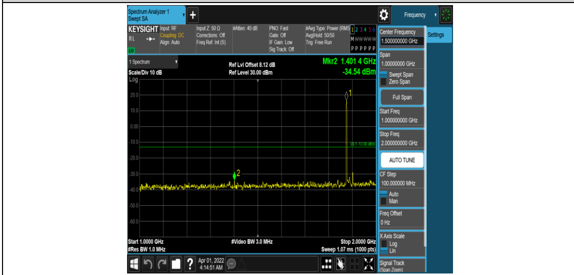
Band25-15MHz-16QAM-26365-1RB#0-Range4:1000~2000MHz
