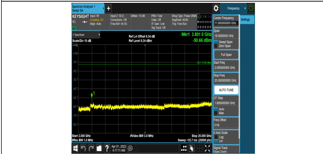
Band25-15MHz-16QAM-26615-1RB#0-Range5:2000~20000MHz
