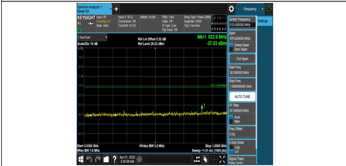
Band25-5MHz-16QAM-26065-1RB#0-Range3:30~1000MHz
