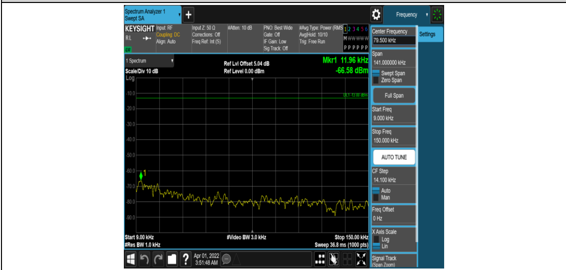
Band25-10MHz-QPSK-26365-1RB#0-Range1:0.009~0.15MHz
