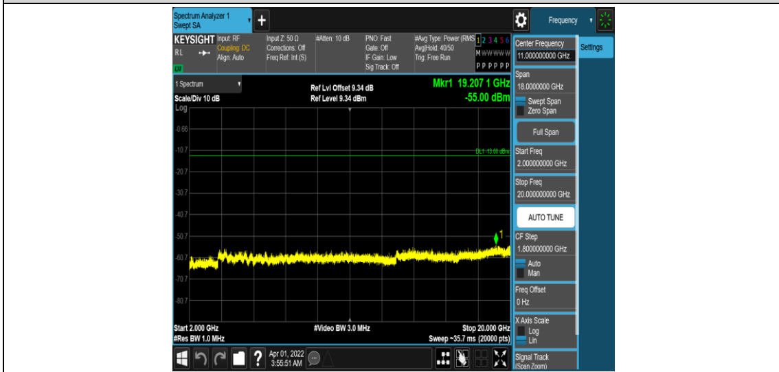
Band25-10MHz-16QAM-26640-1RB#0-Range5:2000~20000MHz
