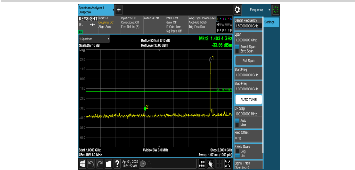
Band25-10MHz-16QAM-26090-1RB#0-Range4:1000~2000MHz
