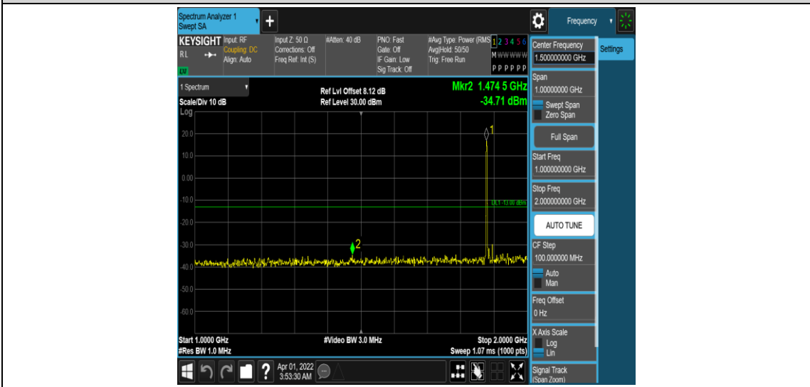
Band25-10MHz-16QAM-26365-1RB#0-Range4:1000~2000MHz
