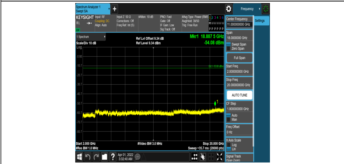
Band25-5MHz-16QAM-26365-1RB#0-Range5:2000~20000MHz
