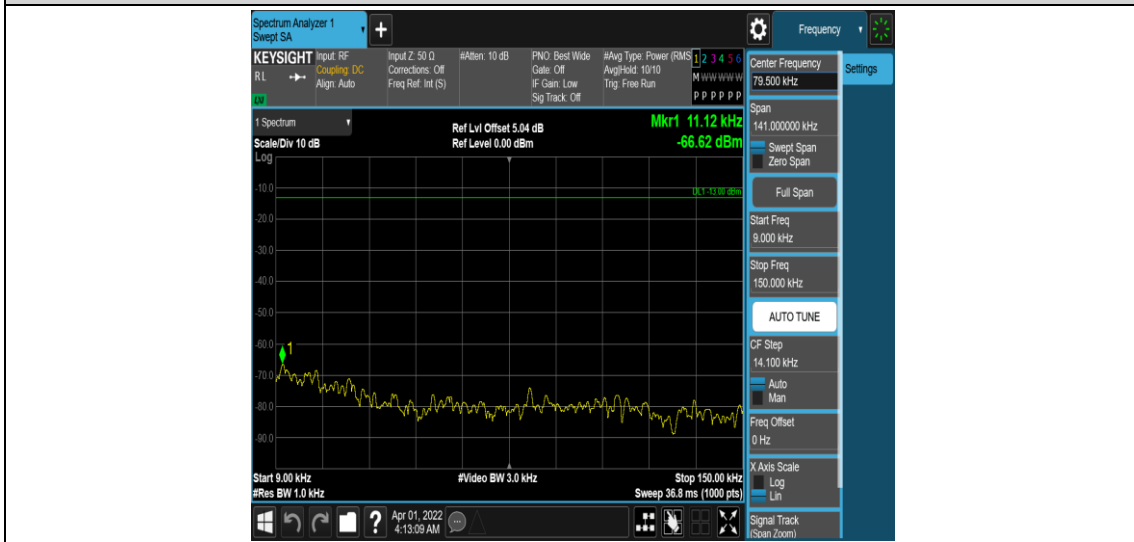
Band25-15MHz-QPSK-26365-1RB#0-Range1:0.009~0.15MHz
