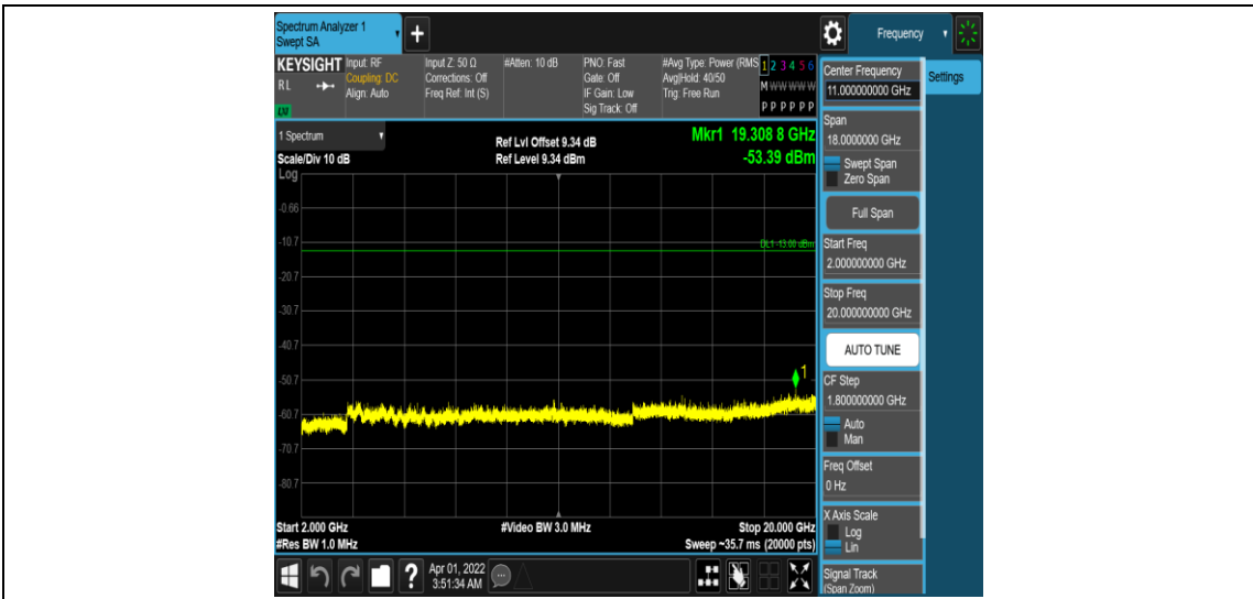
Band25-10MHz-16QAM-26090-1RB#0-Range5:2000~20000MHz
