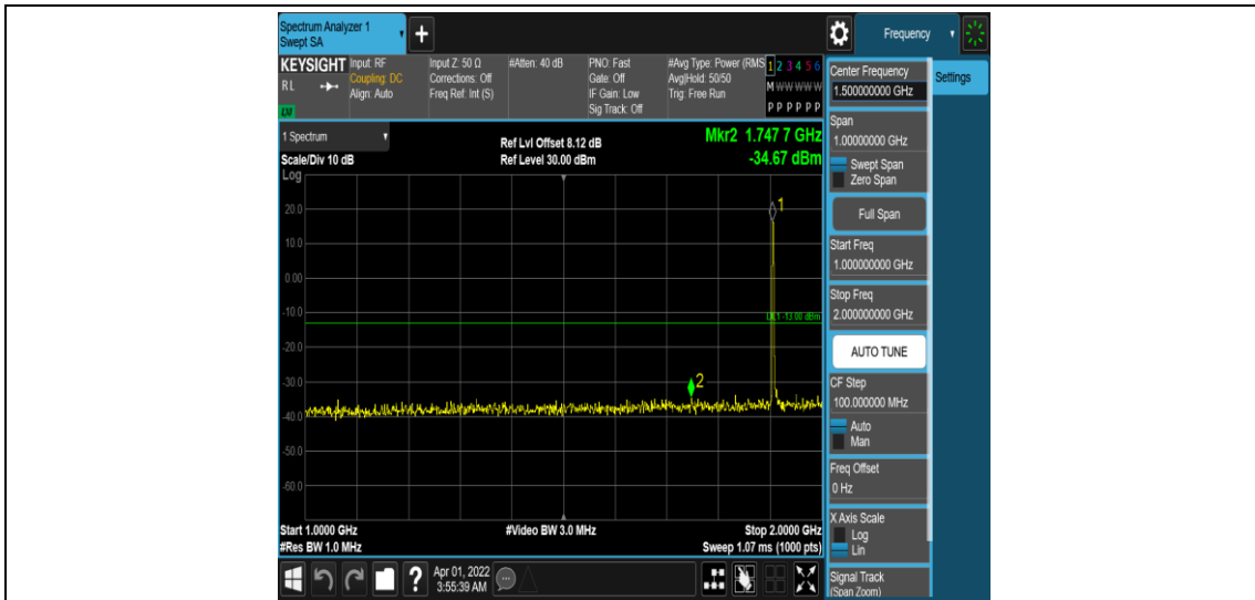
Band25-10MHz-16QAM-26640-1RB#0-Range4:1000~2000MHz
