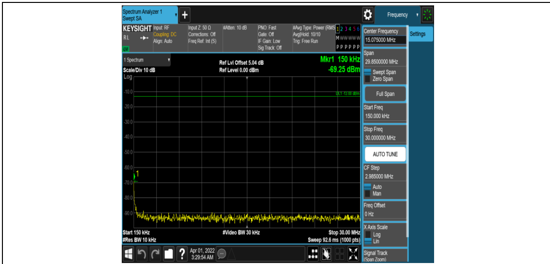
Band25-5MHz-16QAM-26065-1RB#0-Range2:0.15~30MHz
