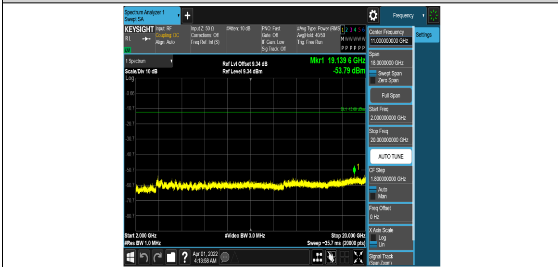
Band25-15MHz-QPSK-26365-1RB#0-Range5:2000~20000MHz
