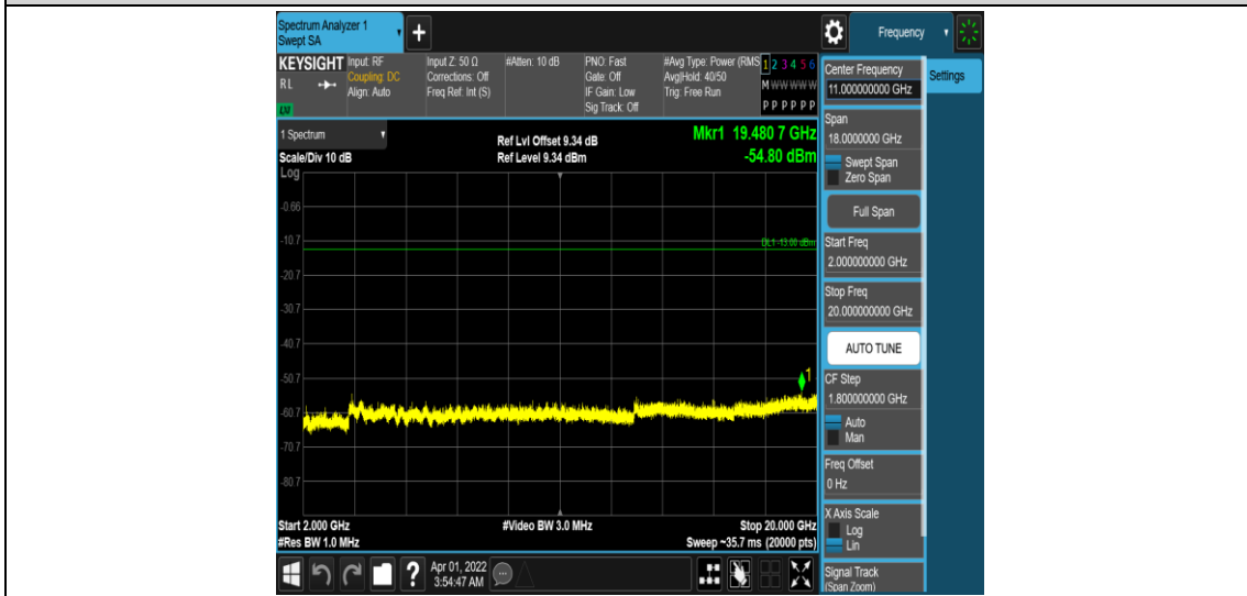
Band25-10MHz-QPSK-26640-1RB#0-Range5:2000~20000MHz
