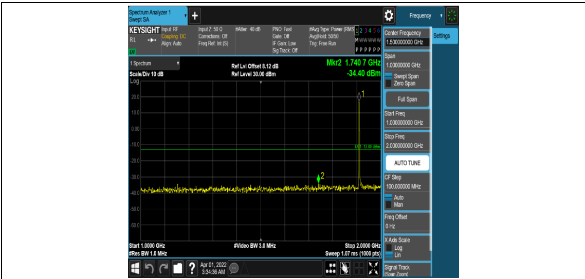
Band25-5MHz-16QAM-26665-1RB#0-Range4: 1000~2000MHz
