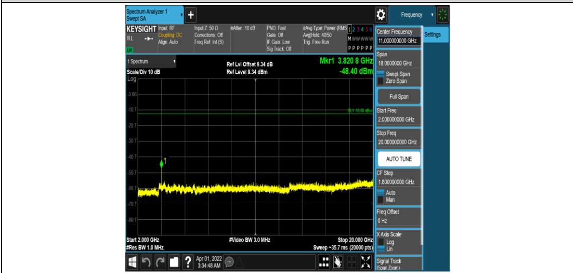
Band25-5MHz-16QAM-26665-1RB#0-Range5:2000~20000MHz
