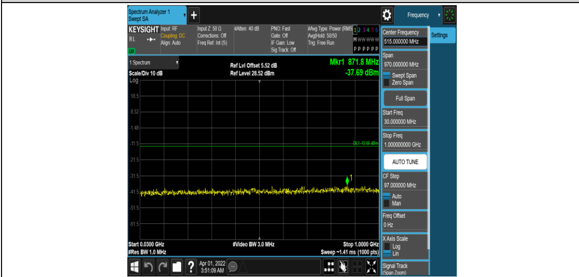
Band25-10MHz-16QAM-26090-1RB#0-Range3:30~1000MHz
