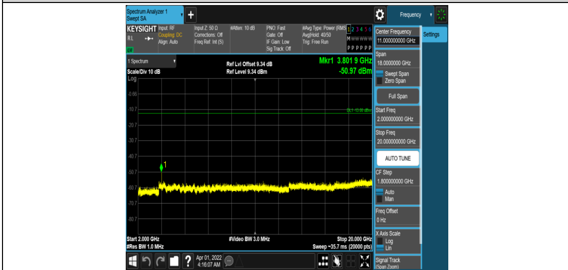
Band25-15MHz-QPSK-26615-1RB#0-Range5:2000~20000MHz
