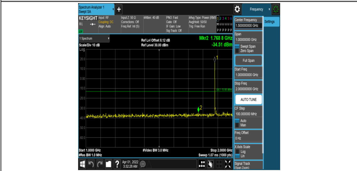
Band25-5MHz-16QAM-26365-1RB#0-Range4:1000~2000MHz
