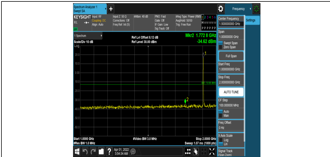
Band25-10MHz-QPSK-26640-1RB#0-Range4:1000~2000MHz
