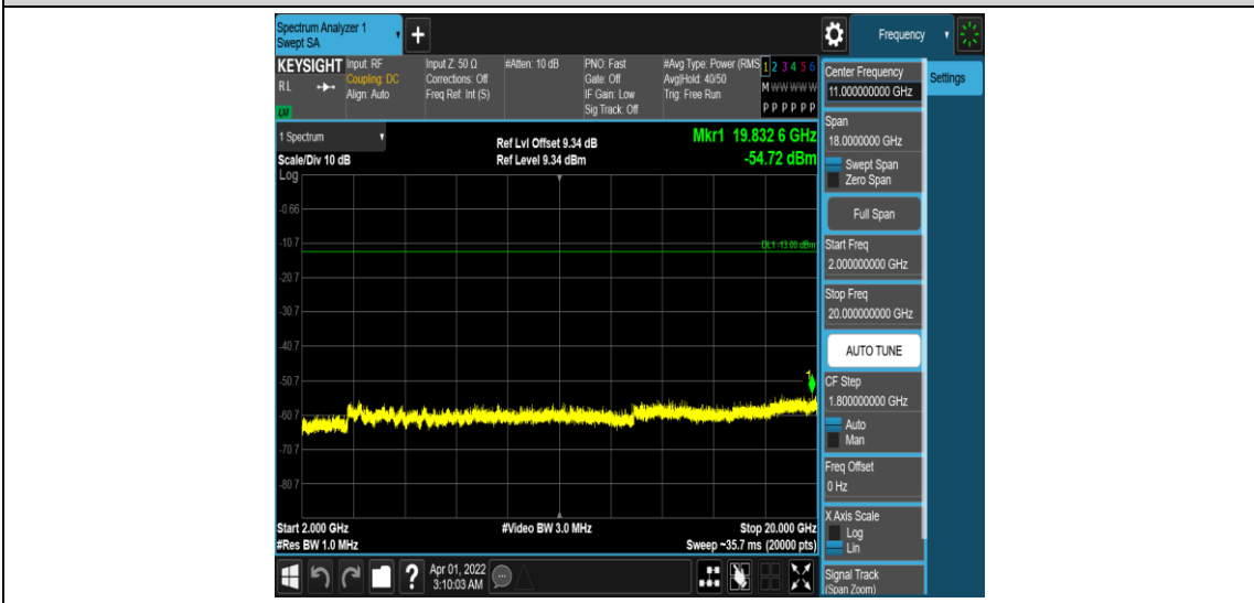
Band25-3MHz-16QAM-26365-1RB#0-Range5:2000~20000MHz
