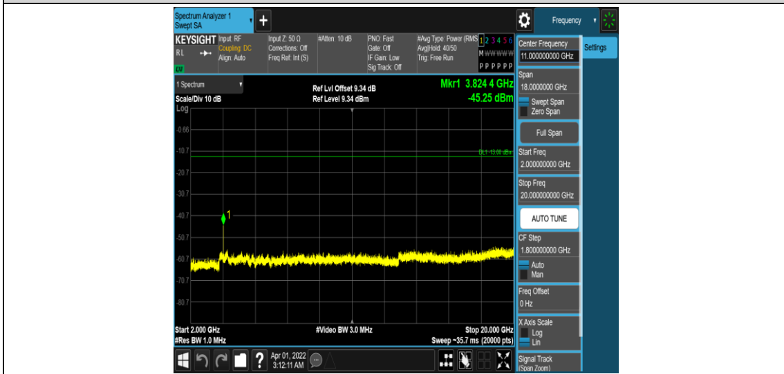
Band25-3MHz-16QAM-26675-1RB#0-Range5:2000~20000MHz
