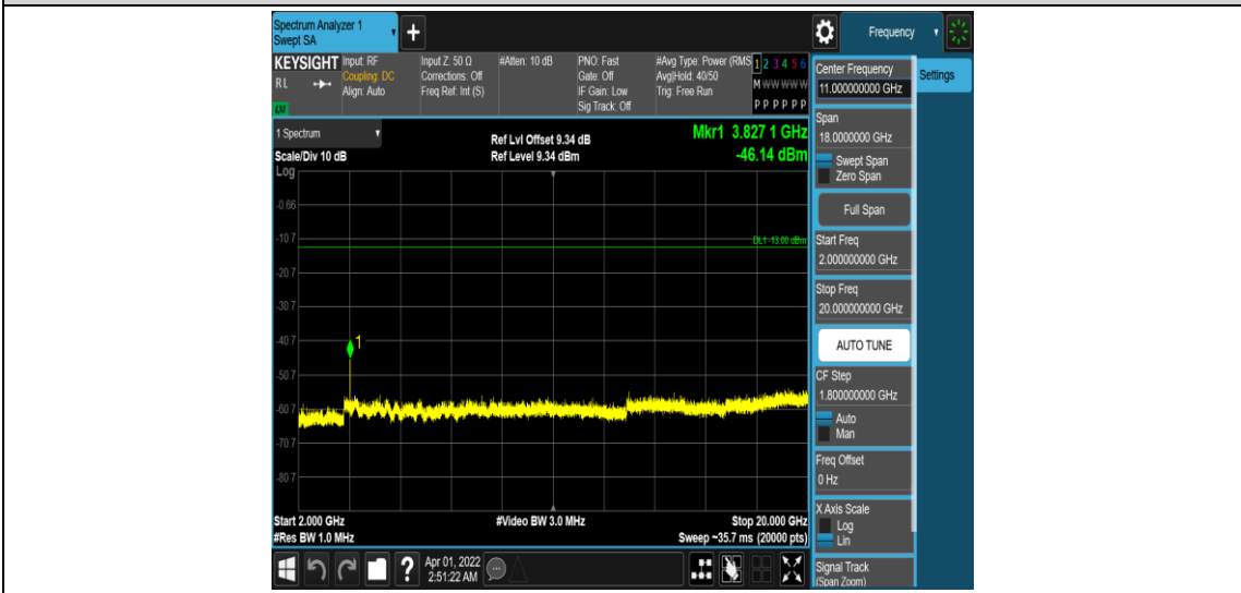
Band25-1.4MHz-16QAM-26683-1RB#0-Range5:2000~20000MHz
