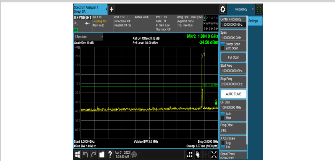
Band25-3MHz-16QAM-26365-1RB#0-Range4:1000~2000MHz
