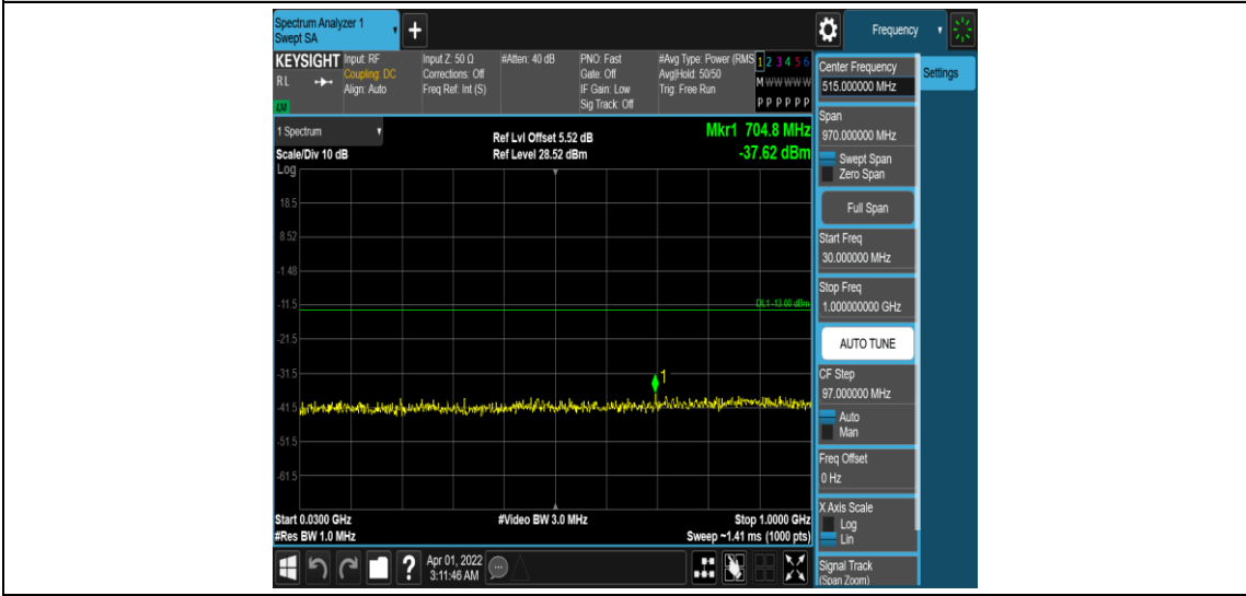
Band25-3MHz-16QAM-26675-1RB#0-Range3:30~1000MHz
