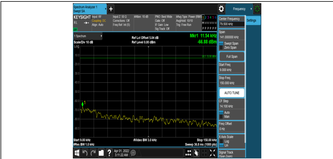
Band25-3MHz-16QAM-26675-1RB#0-Range1:0.009~0.15MHz
