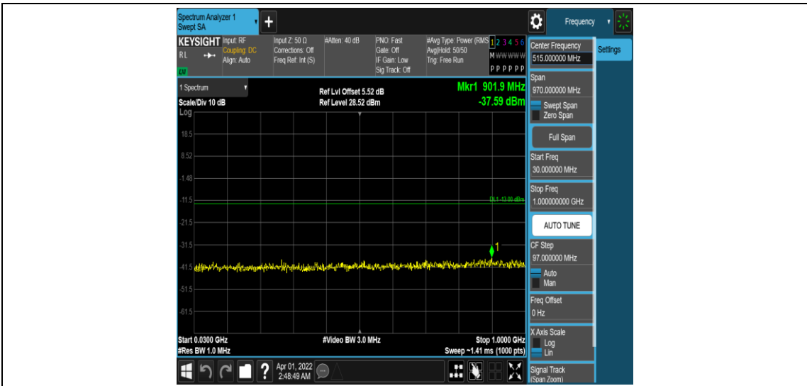
Band25-1.4MHz-16QAM-26365-1RB#0-Range3:30~1000MHz
