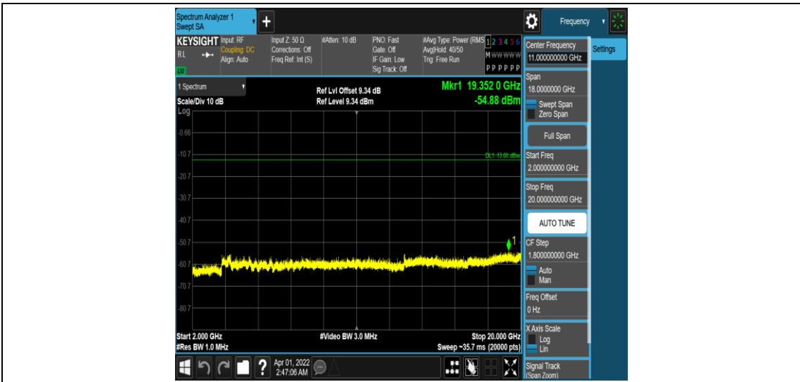
Band25-1.4MHz-16QAM-26047-1RB#0-Range5:2000~20000MHz
