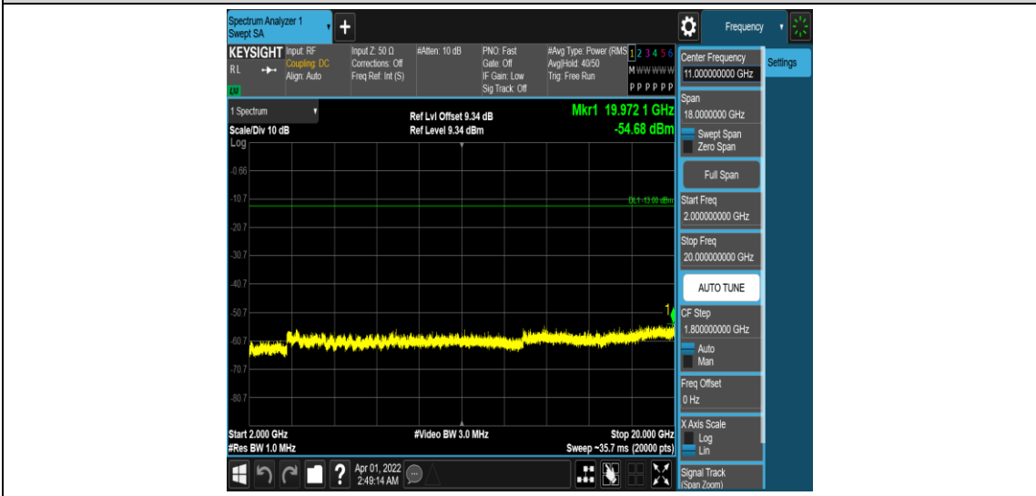
Band25-1.4MHz-16QAM-26365-1RB#0-Range5:2000~20000MHz
