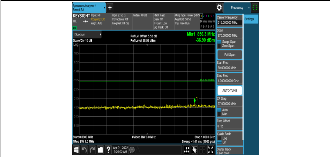
Band25-5MHz-QPSK-26065-1RB#0-Range3:30~1000MHz
