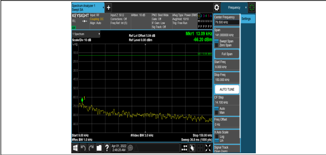
Band25-1.4MHz-16QAM-26365-1RB#0-Range1:0.009~0.15MHz
