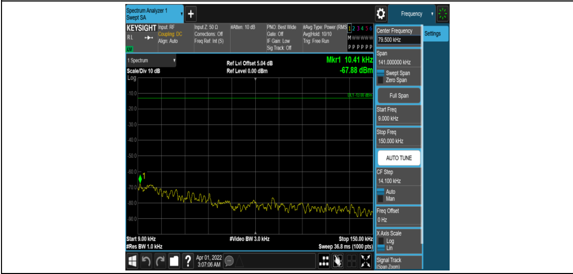
Band25-3MHz-16QAM-26055-1RB#0-Range1:0.009~0.15MHz
