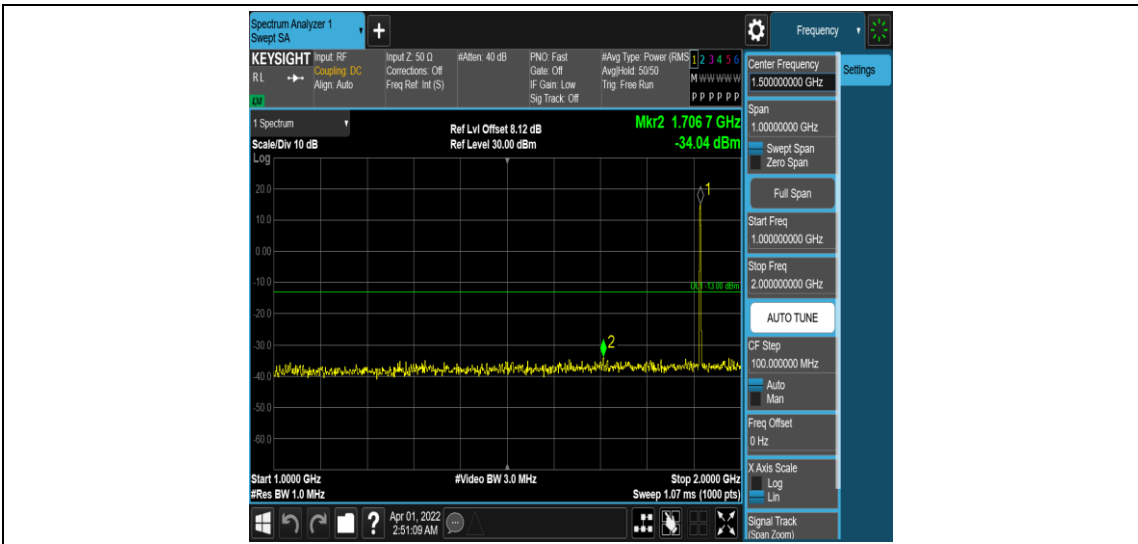
Band25-1.4MHz-16QAM-26683-1RB#0-Range4:1000~2000MHz
