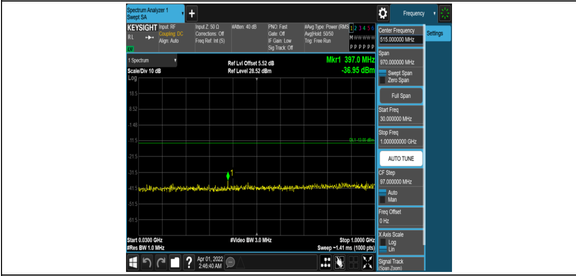
Band25-1.4MHz-16QAM-26047-1RB#0-Range3:30~1000MHz
