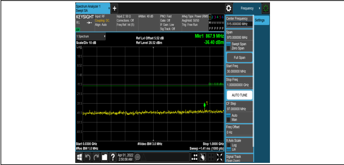
Band25-1.4MHz-16QAM-26683-1RB#0-Range3:30~1000MHz
