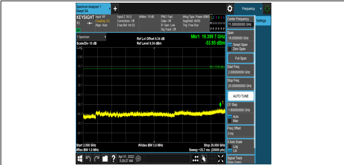
Band25-5MHz-QPSK-26065-1RB#0-Range5:2000~20000MHz
