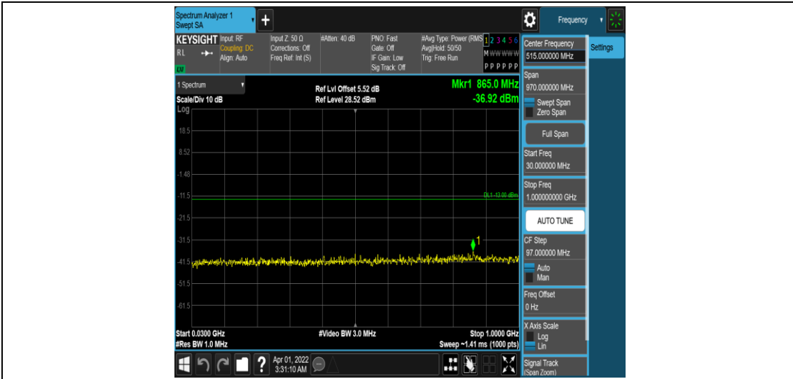
Band25-5MHz-QPSK-26365-1RB#0-Range3:30~1000MHz
