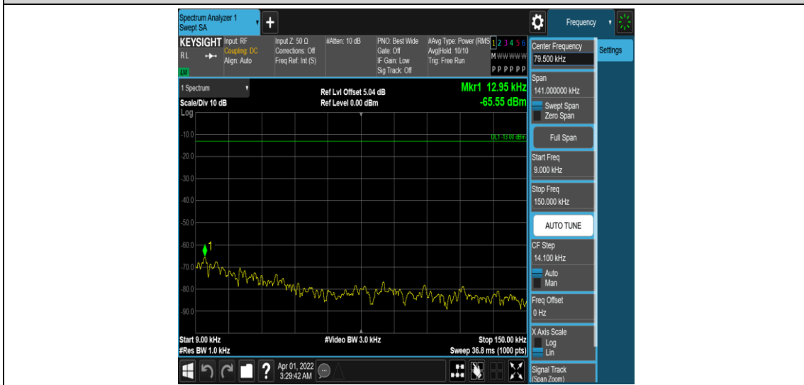
Band25-5MHz-16QAM-26065-1RB#0-Range1:0.009~0.15MHz
