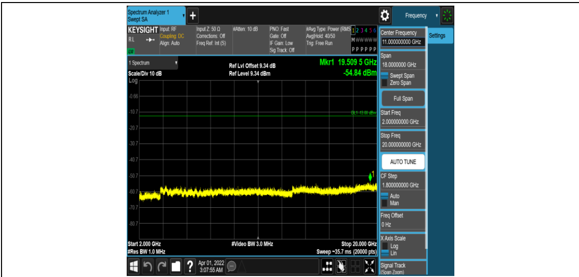
Band25-3MHz-16QAM-26055-1RB#0-Range5:2000~20000MHz
