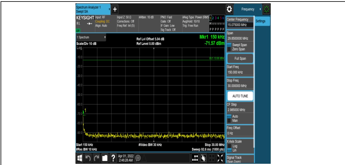
Band25-1.4MHz-16QAM-26047-1RB#0-Range2:0.15~30MHz
