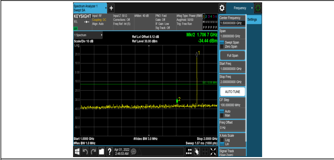
Band25-1.4MHz-16QAM-26047-1RB#0-Range4:1000~2000MHz
