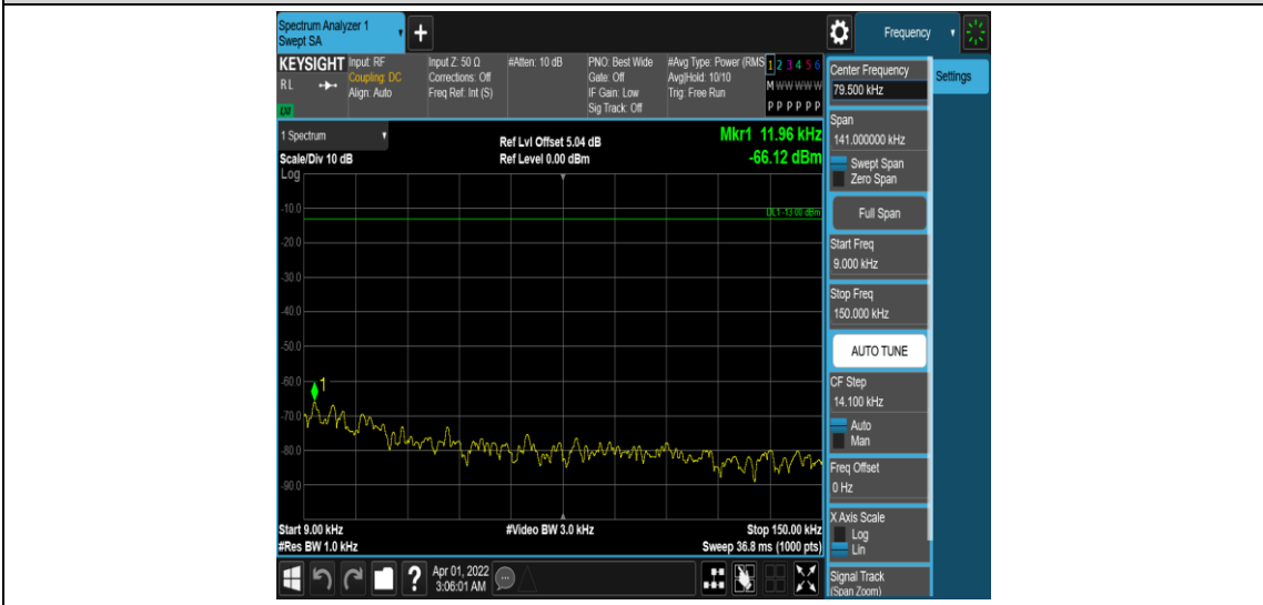
Band25-3MHz-QPSK-26055-1RB#0-Range1:0.009~0.15MHz
