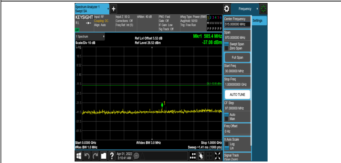
Band25-3MHz-QPSK-26675-1RB#0-Range3:30~1000MHz
