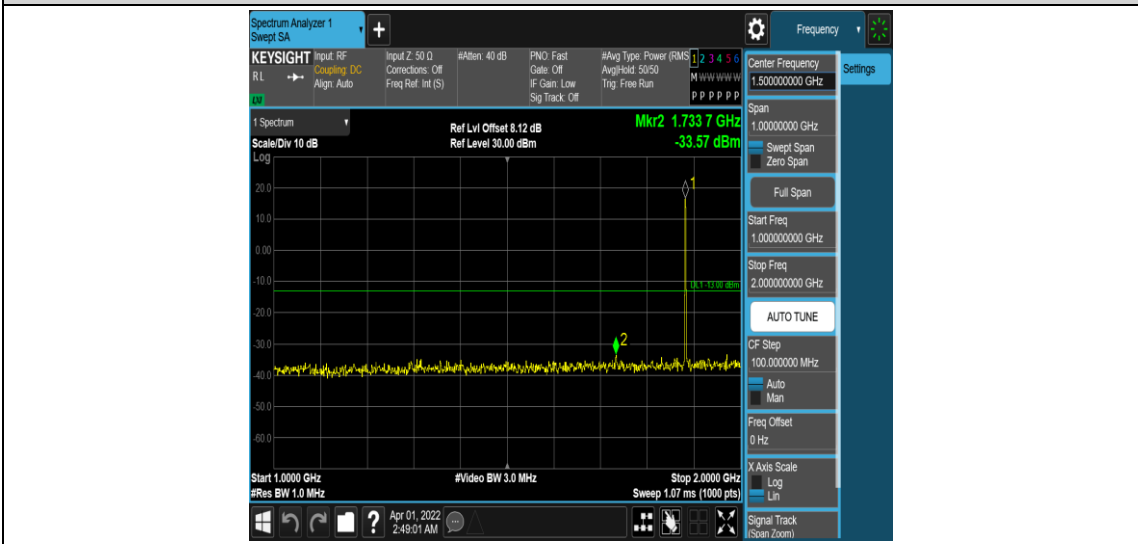
Band25-1.4MHz-16QAM-26365-1RB#0-Range4:1000~2000MHz
