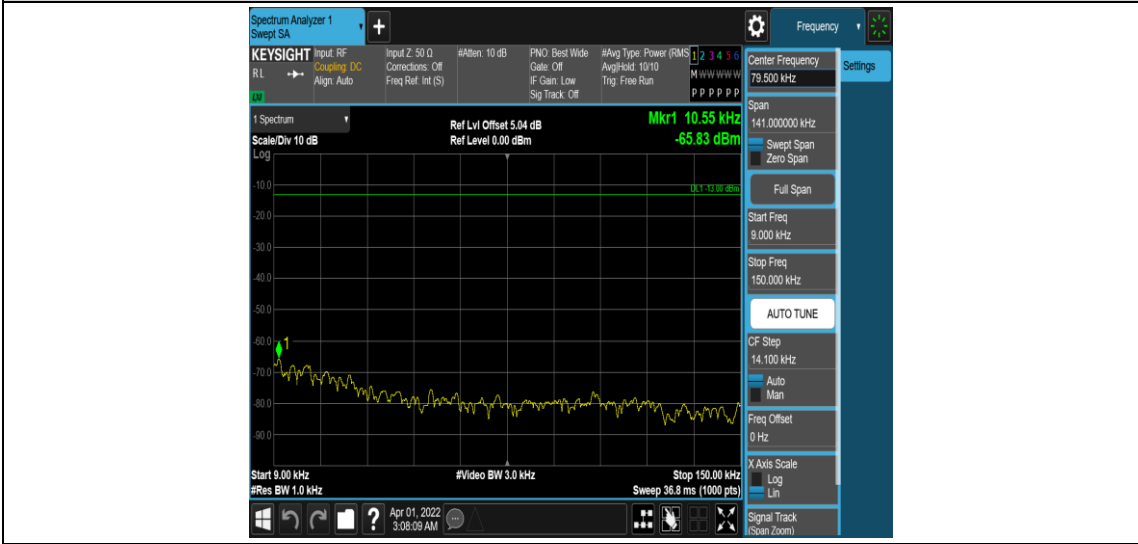
Band25-3MHz-QPSK-26365-1RB#0-Range1:0.009~0.15MHz
