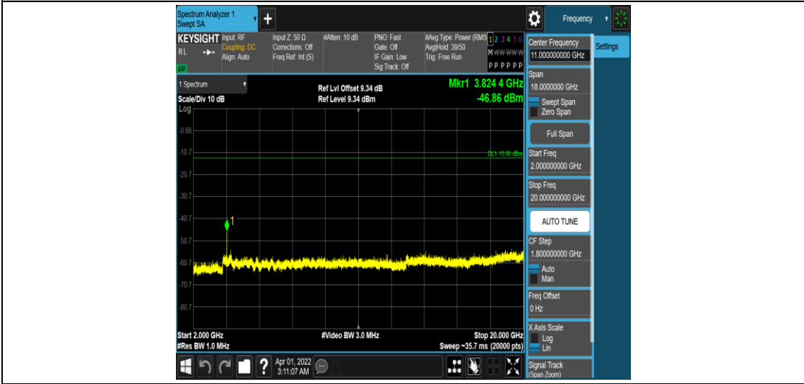
Band25-3MHz-QPSK-26675-1RB#0-Range5:2000~20000MHz
