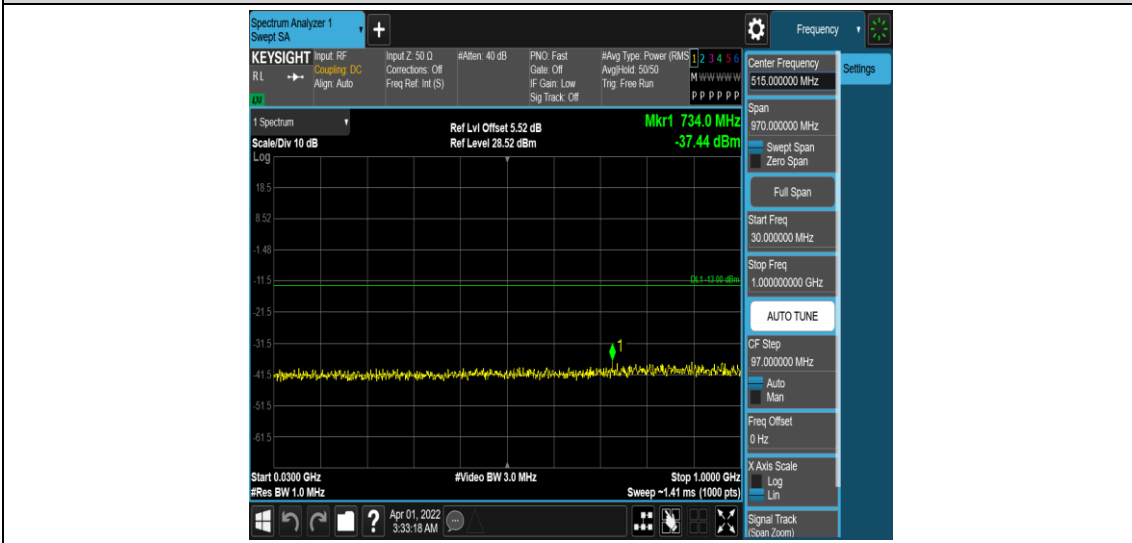
Band25-5MHz-QPSK-26665-1RB#0-Range3:30~1000MHz
