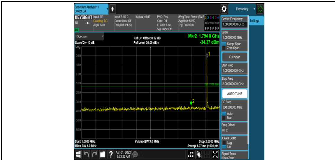
Band25-5MHz-QPSK-26665-1RB#0-Range4:1000~2000MHz
