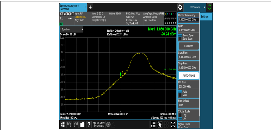
Band25-5MHz-16QAM-26065-1RB#0
