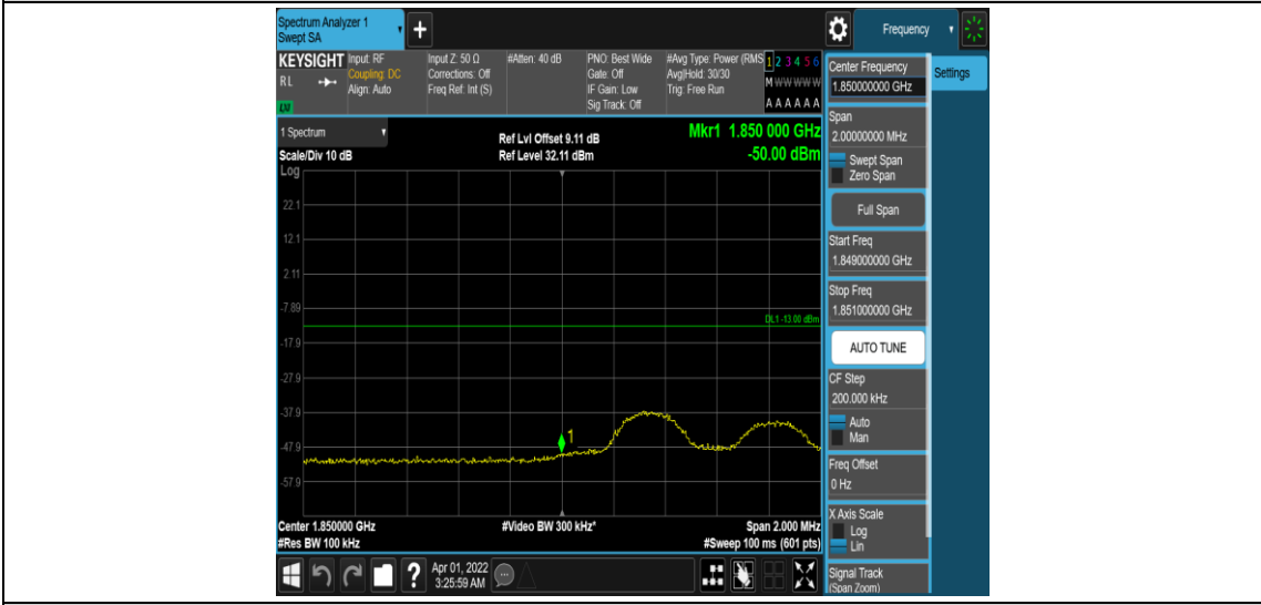
Band25-5MHz-16QAM-26065-1RB#24
