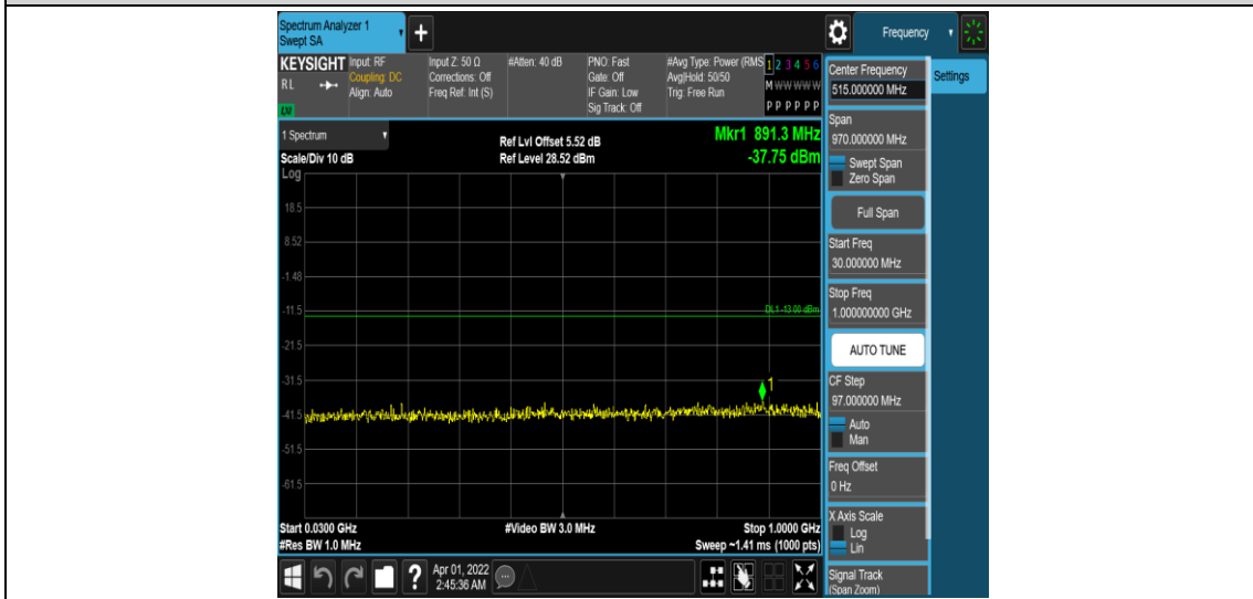
Band25-1.4MHz-QPSK-26047-1RB#0-Range3:30~1000MHz
