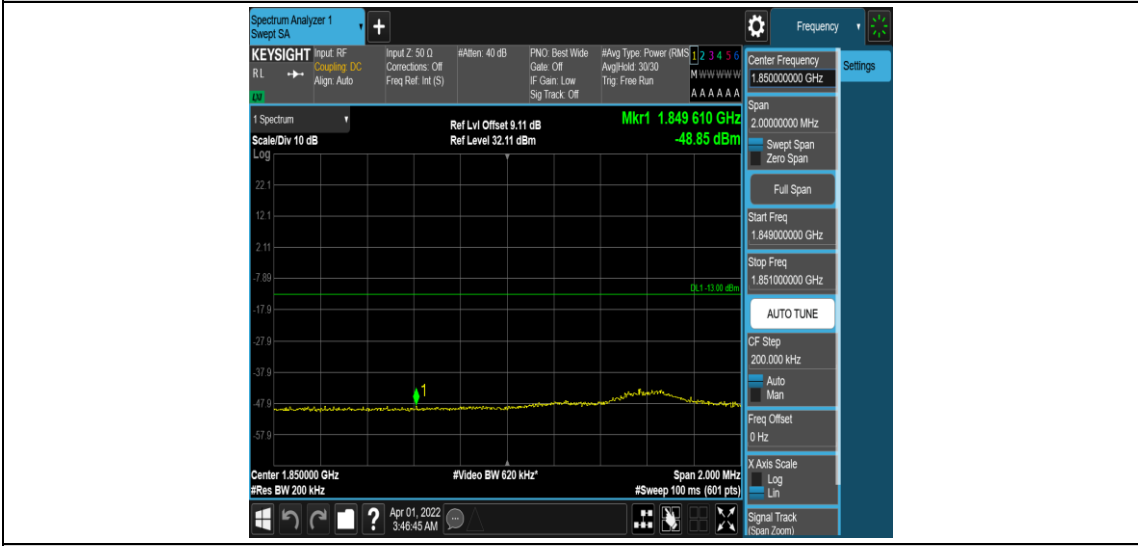
Band25-10MHz-QPSK-26090-1RB#49
