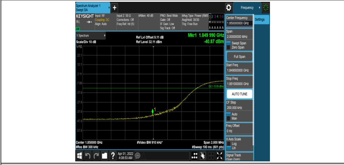
Band25-15MHz-16QAM-26115-75RB#0
