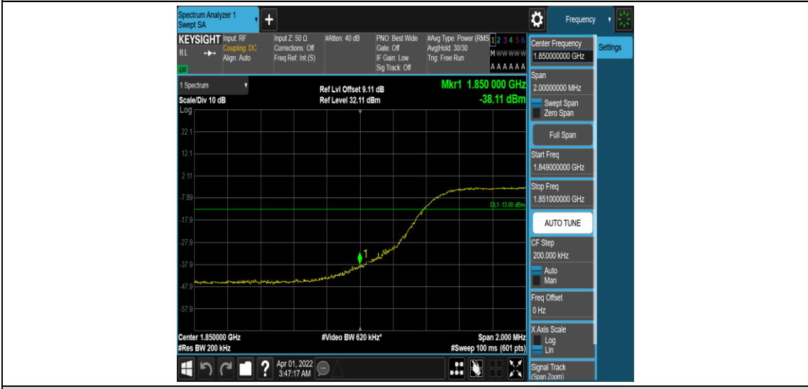
Band25-10MHz-QPSK-26090-50RB#0
