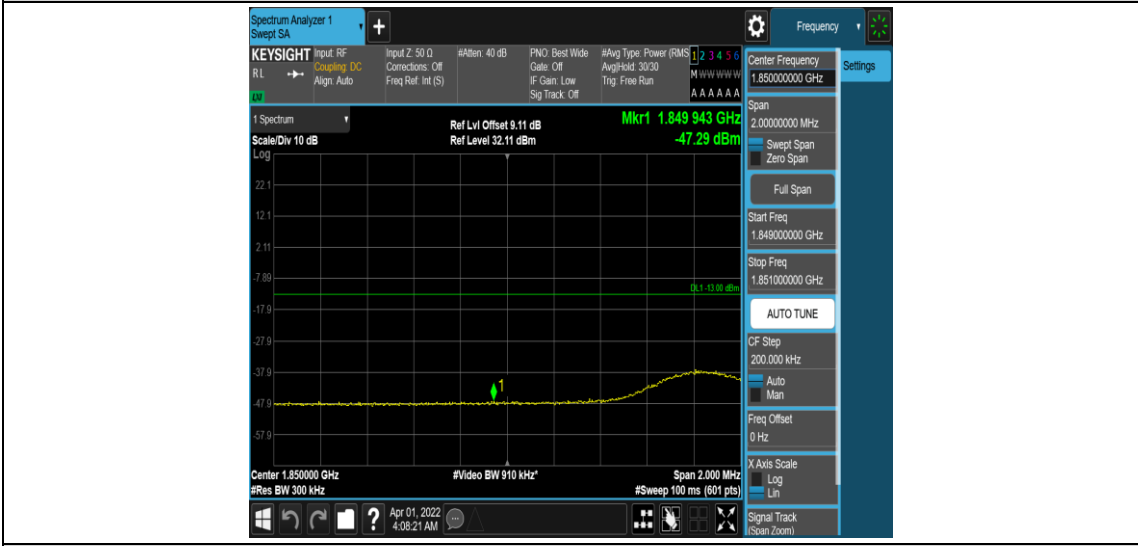
Band25-15MHz-16QAM-26115-1RB#74
