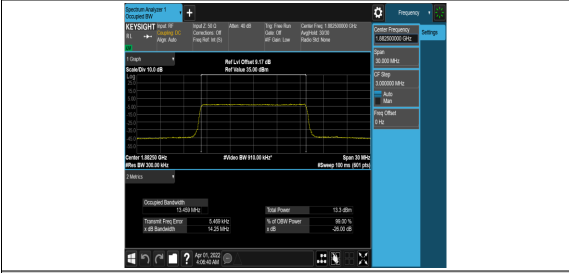
Band25-15MHz-16QAM-26365-75RB#0
