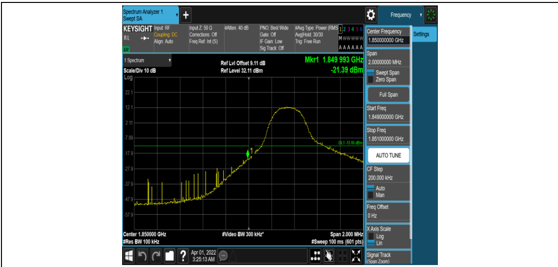
Band25-5MHz-QPSK-26065-1RB#0
