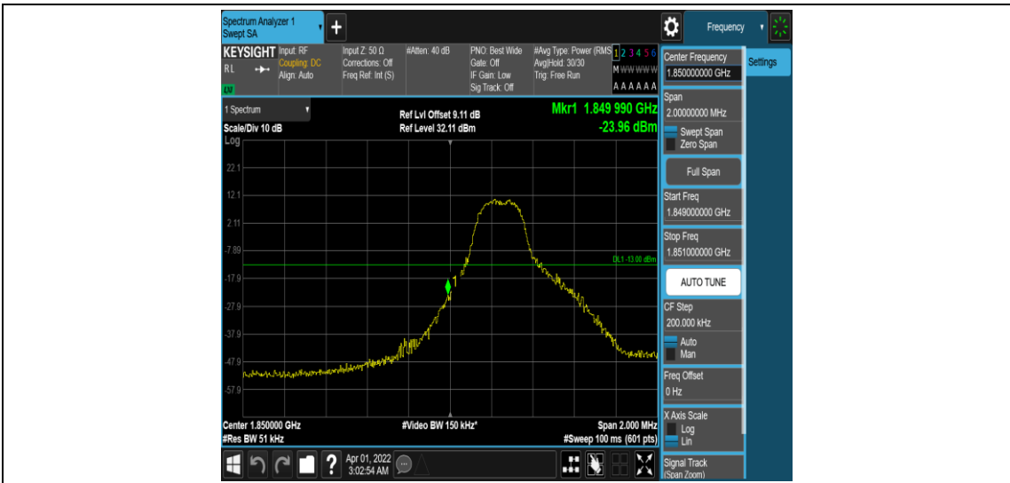
Band25-3MHz-16QAM-26055-1RB#0
