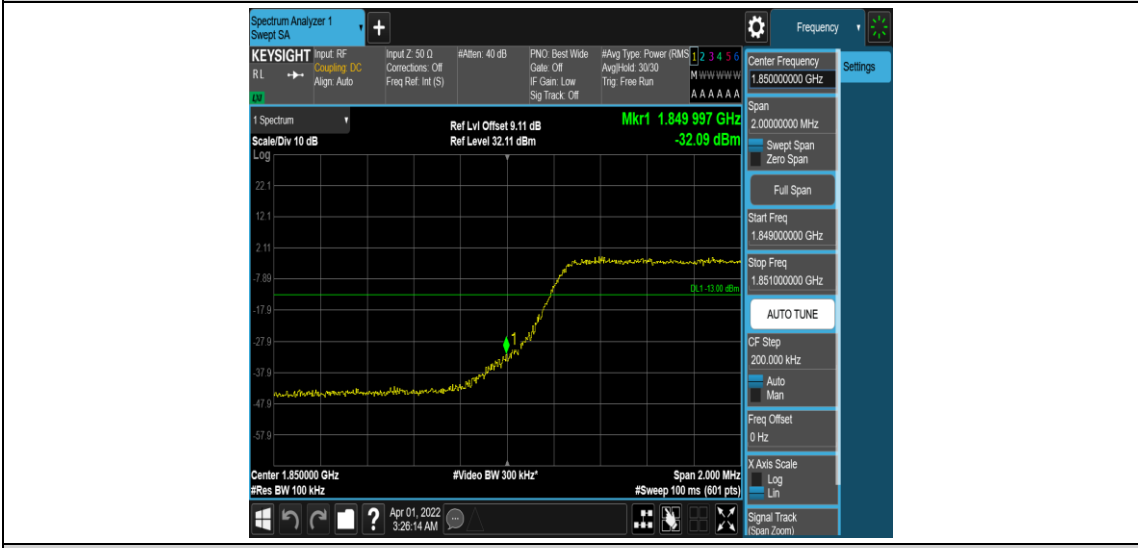
Band25-5MHz-QPSK-26065-25RB#0
