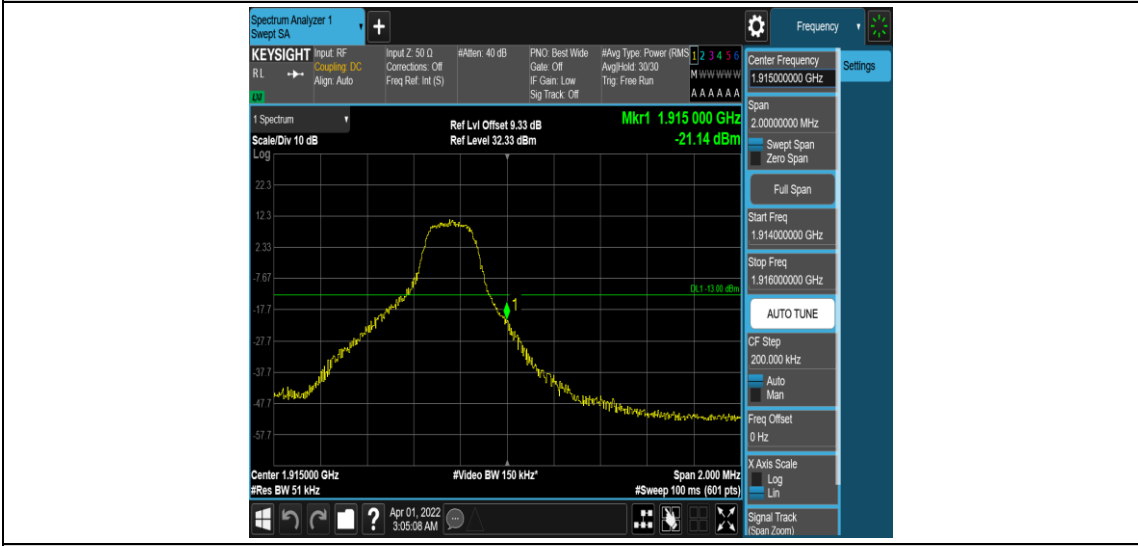
Band25-3MHz-16QAM-26675-1RB#14
