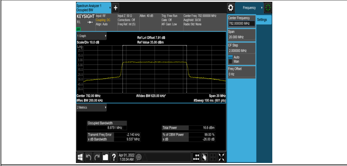
Band13-10MHz-16QAM-23230-50RB#0
