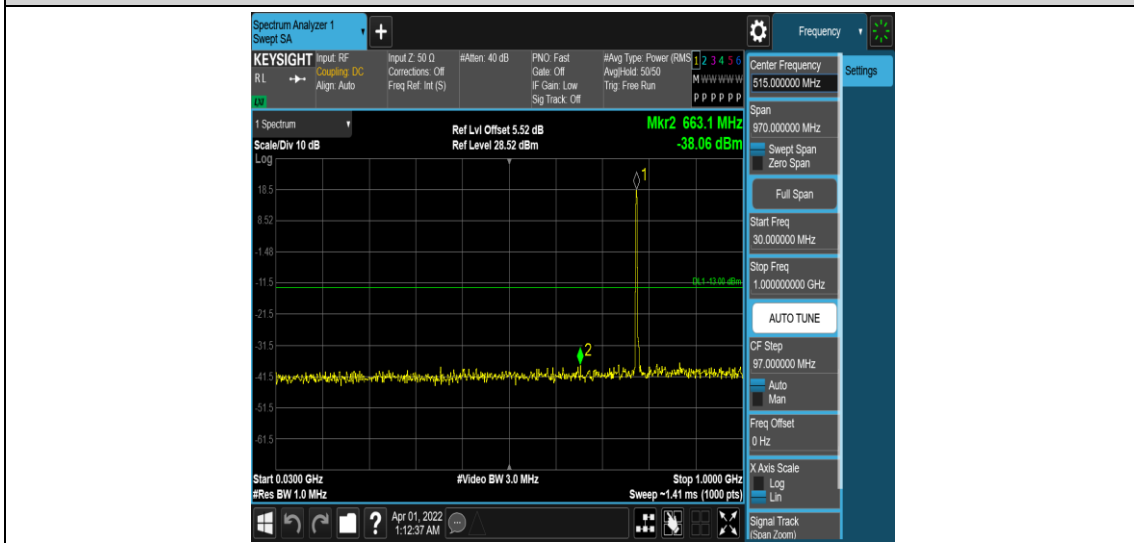
Band13-5MHz-QPSK-23230-1RB#0-Range3:30~1000MHz
