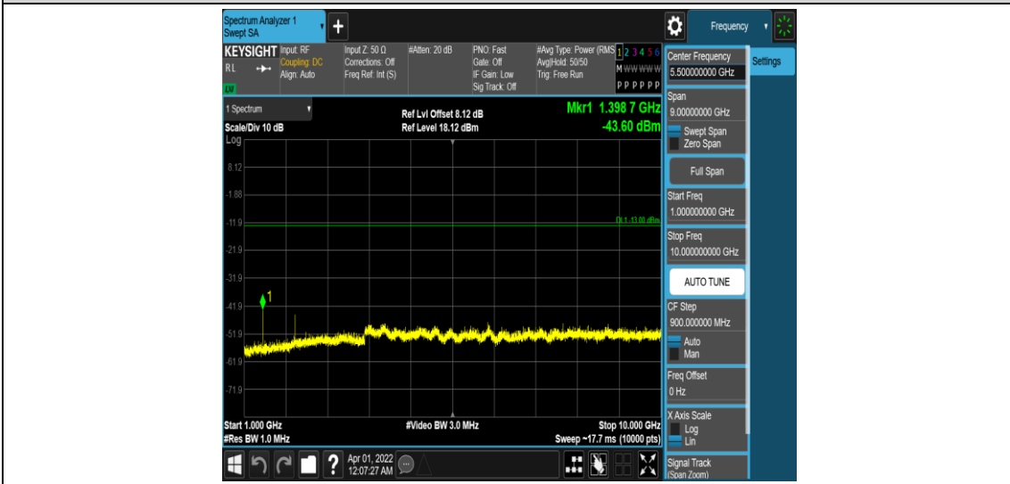
Band12-3MHz-16QAM-23025-1RB#0-Range4:1000~10000MHz
