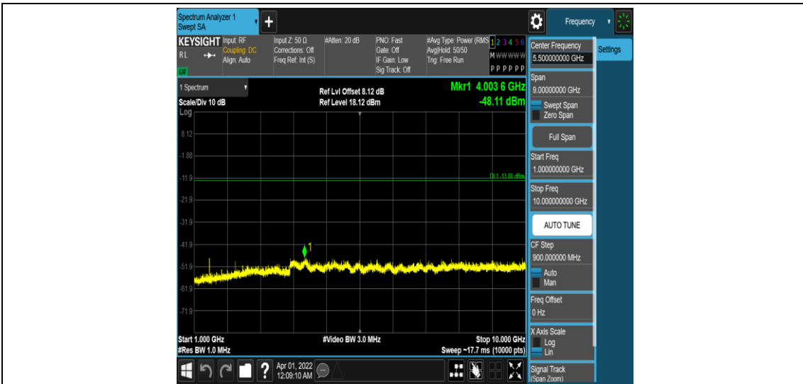
Band12-3MHz-16QAM-23095-1RB#0-Range4:1000~10000MHz
