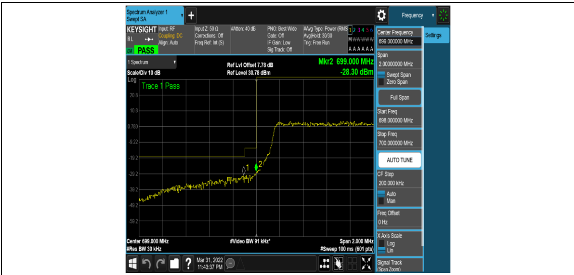
Band12-1.4MHz-16QAM-23017-6RB#0
