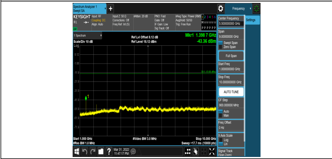
Band12-1.4MHz-16QAM-23017-1RB#0-Range4:1000~10000MHz
