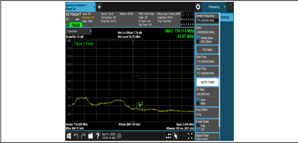
Band12-3MHz-QPSK-23165-1RB#0
