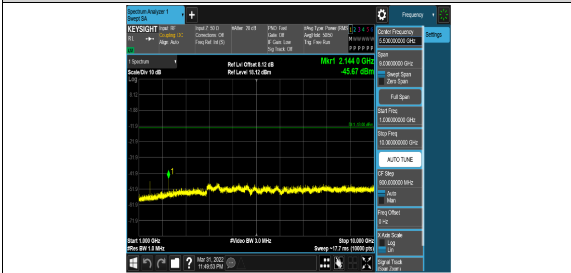
Band12-1.4MHz-QPSK-20173-1RB#0-Range4:1000~10000MHz
