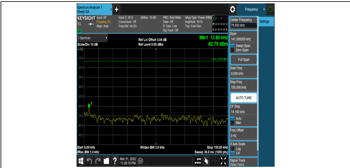
Band5-10MHz-QPSK-20525-1RB#0-Range1:0.009~0.15MHz
