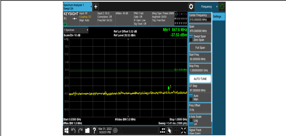
Band4-5MHz-16QAM-19975-1RB#0-Range3:30~100MHz
