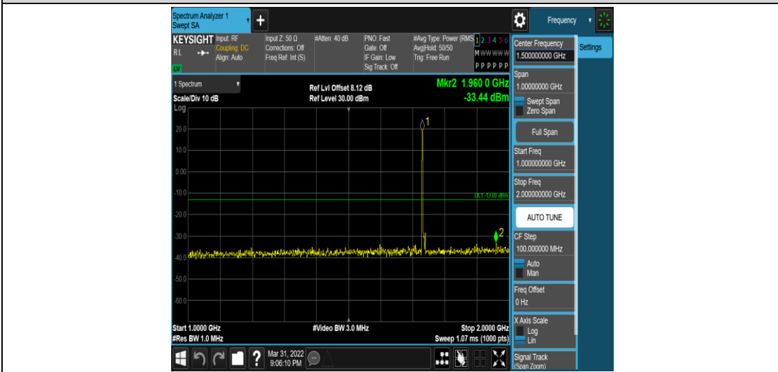
Band4-5MHz-16QAM-20175-1RB#0-Range4:1000~2000MHz
