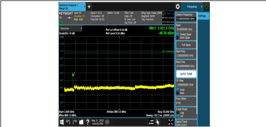
Band4-10MHz-16QAM-2000-1RB#0-Range5:2000~20000MHz
