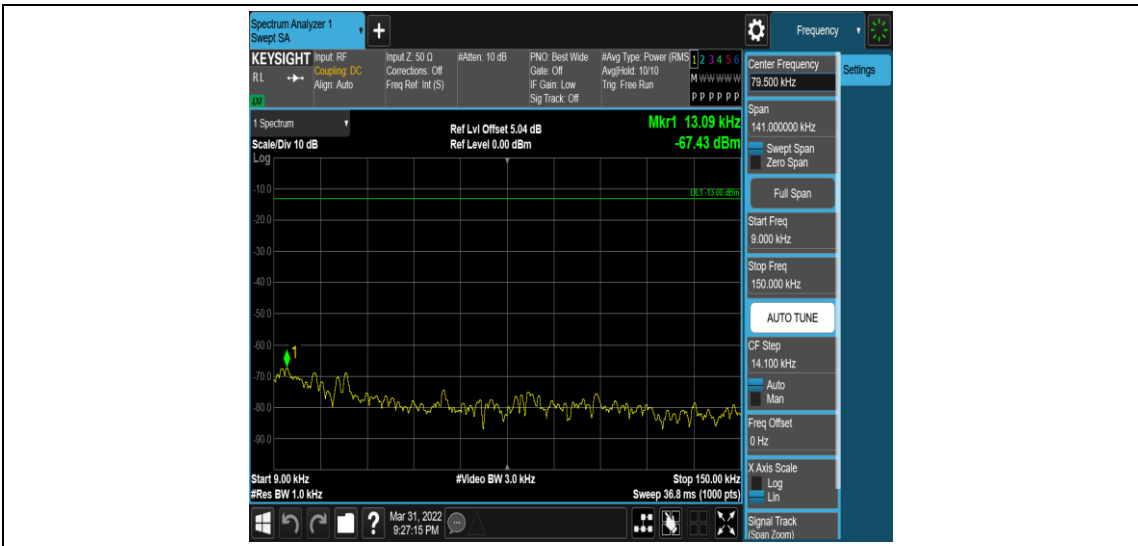
Band4-10MHz-QPSK-20350-1RB#0-Range1:0.009~0.15MHz
