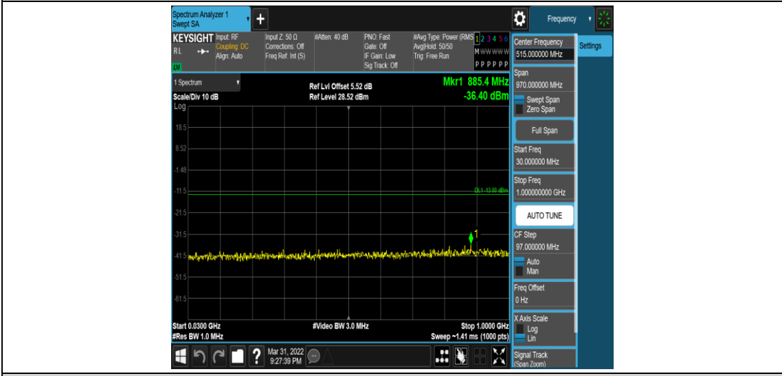
Band4-10MHz-QPSK-20350-1RB#0-Range3:30~1000MHz
