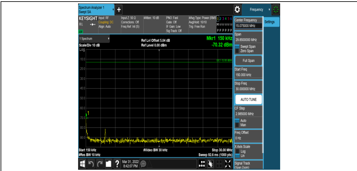
Band4-3MHz-16QAM-19965-1RB#0-Range2:0.15~30MHz
