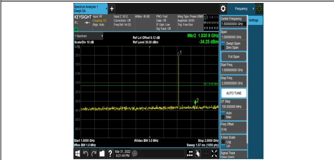
Band4-1.4MHz-16QAM-19957-1RB#0-Range4:1000~2000MHz
