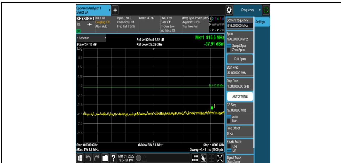
Band4-5MHz-QPSK-20175-1RB#0-Range3:30~1000MHz
