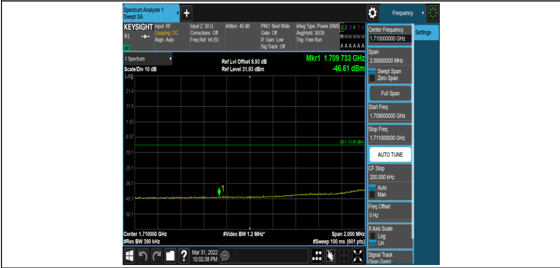
Band4-20MHz-16QAM-20050-1RB#90
