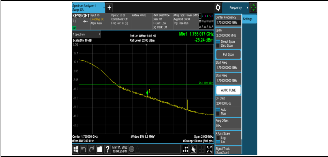
Band4-20MHz-16QAM-20300-1RB#99
