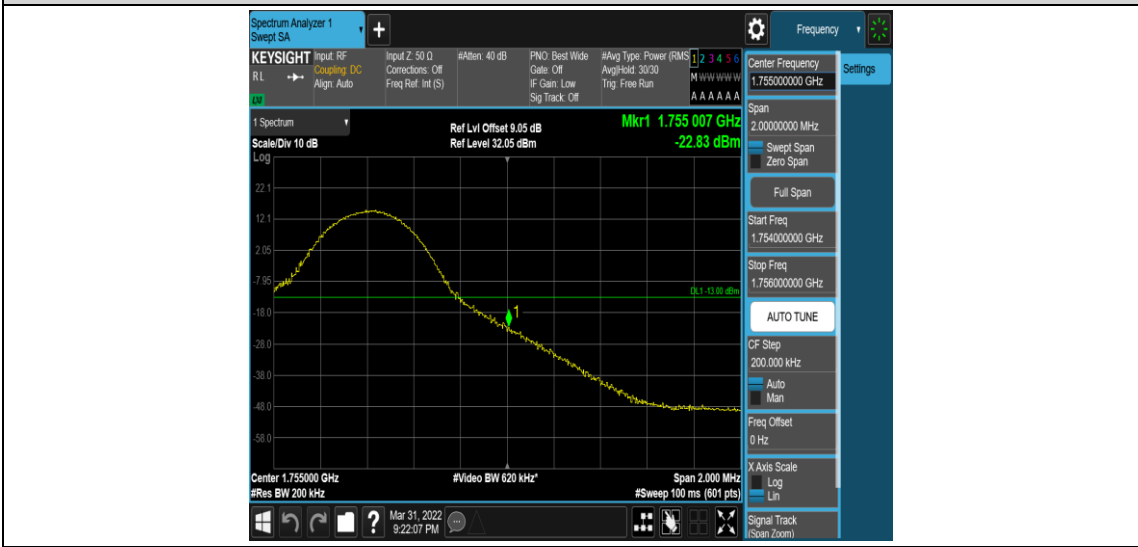
Band4-10MHz-16QAM-20350-1RB#49
