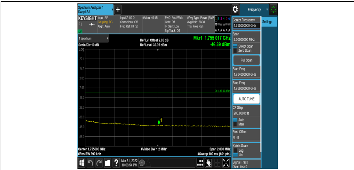
Band4-20MHz-16QAM-20300-1RB#0
