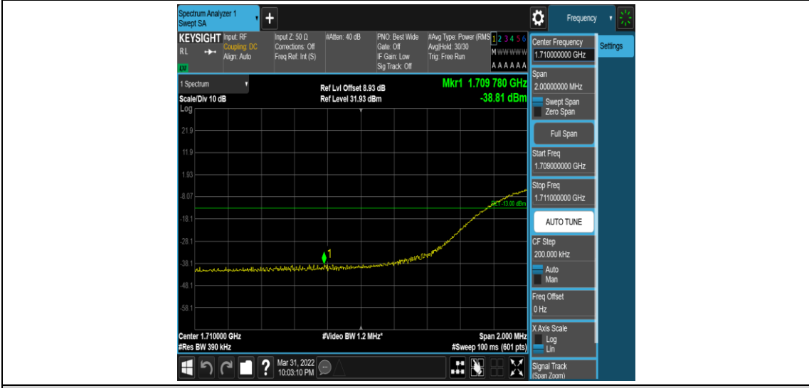
Band4-20MHz-16QAM-20050-100RB#0
