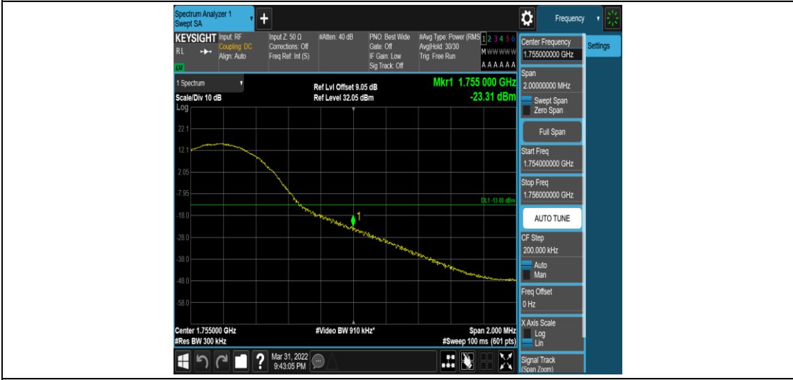
Band4-15MHz-16QAM-20325-1RB#74
