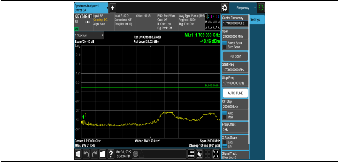
Band4-3MHz-16QAM-19965-1RB#14
