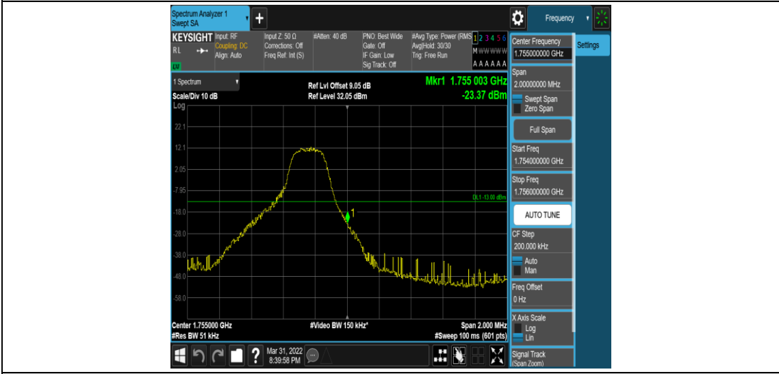
Band4-3MHz-16QAM-20385-1RB#14
