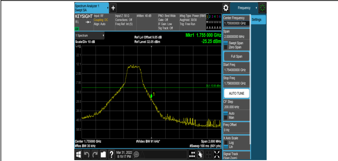
Band4-1.4MHz-16QAM-20393-1RB#5
