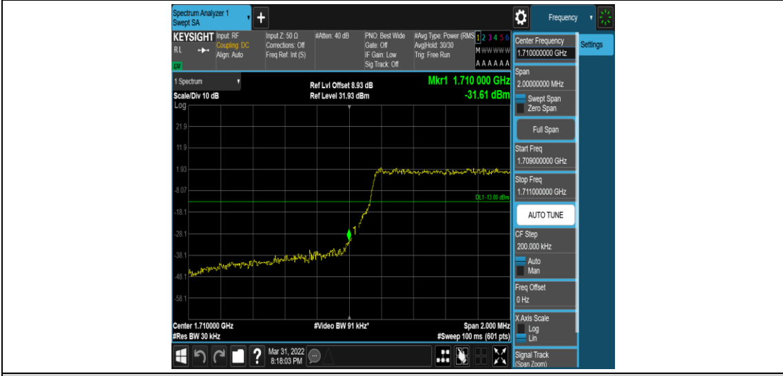
Band4-1.4MHz-16QAM-19957-6RB#0
