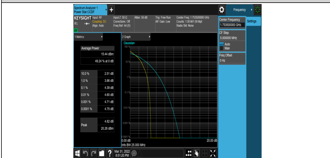
Band4-3MHz-QPSK-20385-1RB#0
