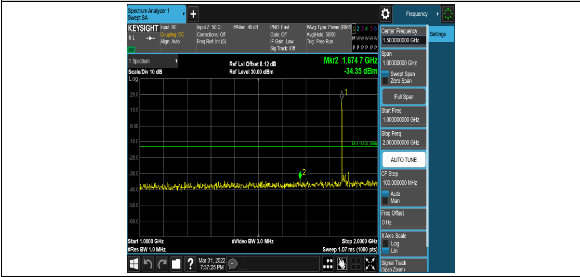
Band2-15MHz-QPSK-18675-1RB#0-Range4:1000~2000MHz
