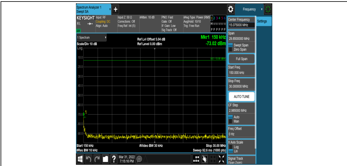
Band2-10MHz-16QAM-18650-1RB#0-Range2:0.15~30MHz
