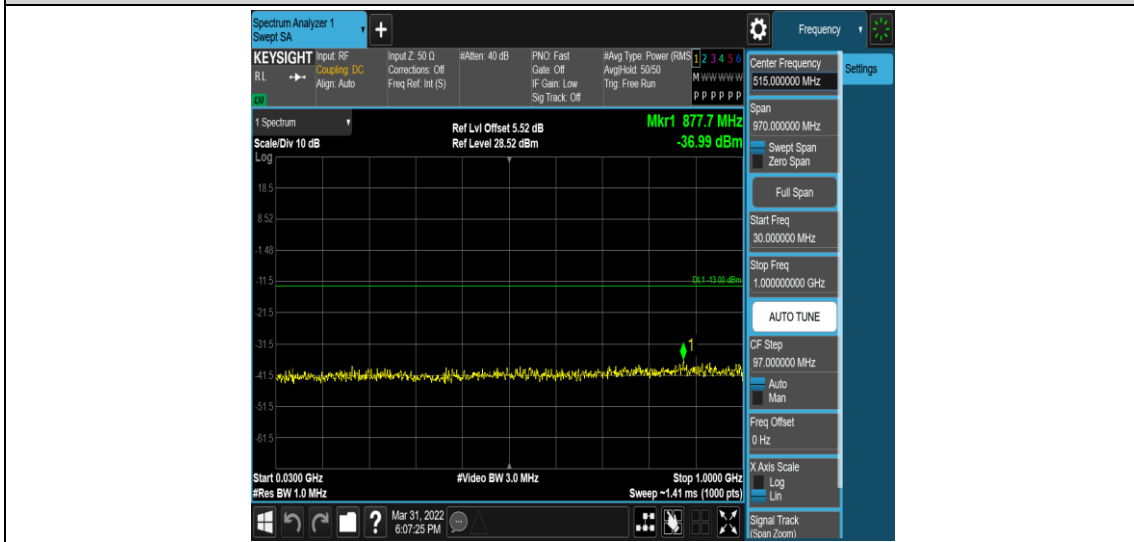
Band2-1.4MHz-16QAM-18607-1RB#0-Range3:30~1000MHz
