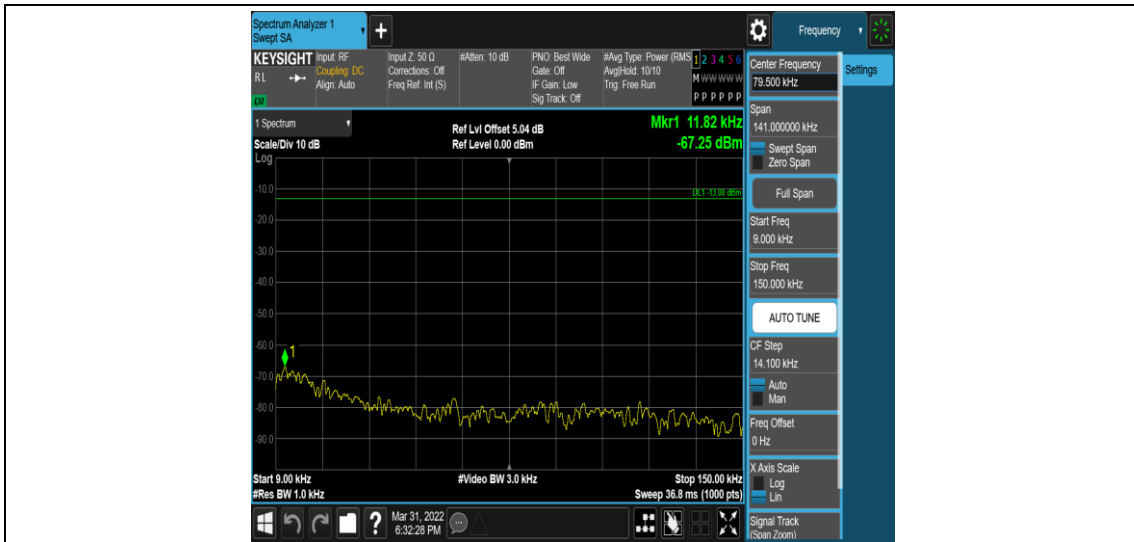
Band2-3MHz-QPSK-19185-1RB#0-Range1:0.009~0.15MHz
