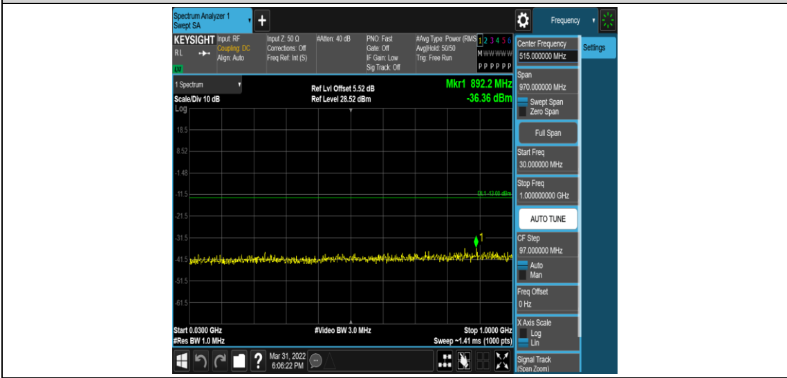
Band2-1.4MHz-QPSK-18607-1RB#0-Range3:30~1000MHz
