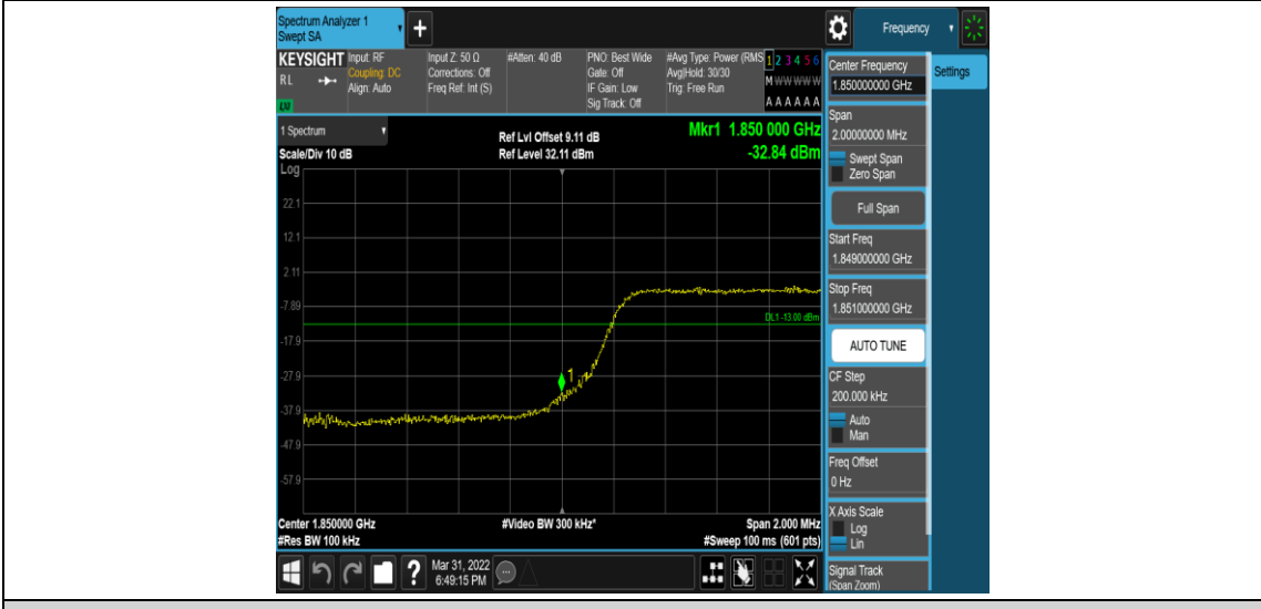
Band2-5MHz-16QAM-18625-25RB#0
