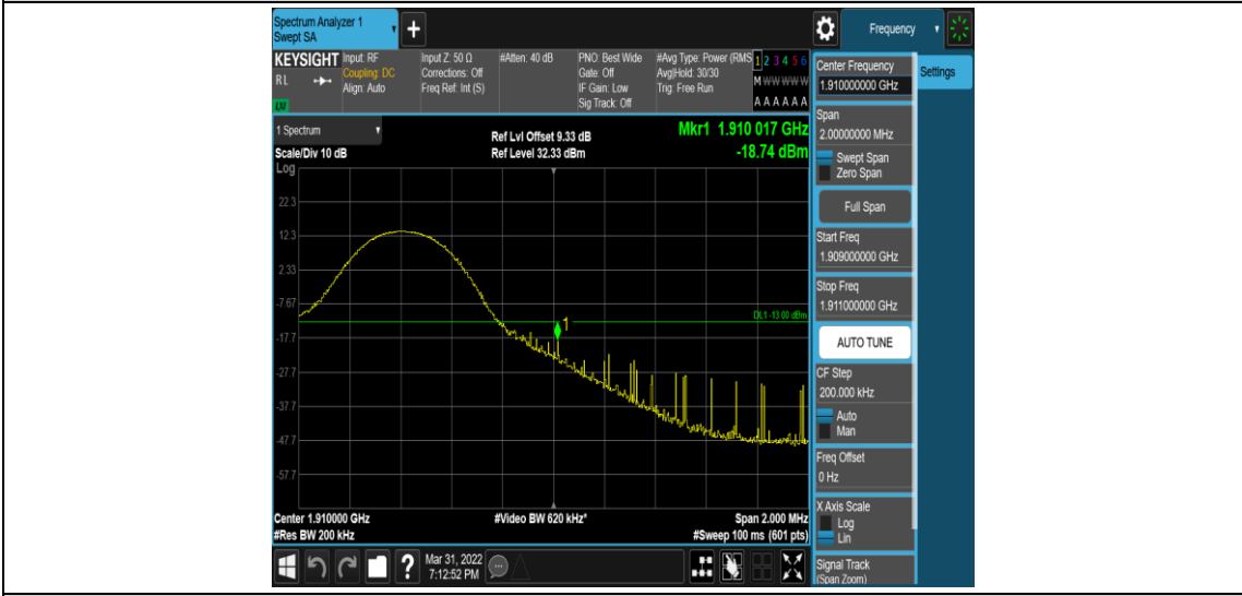
Band2-10MHz-QPSK-19150-1RB#49
