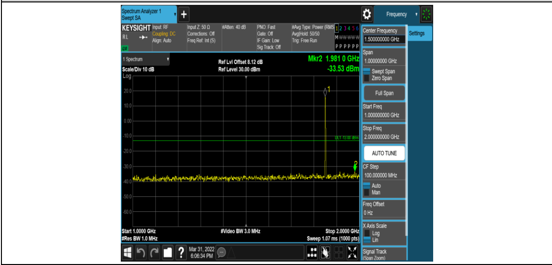
Band2-1.4MHz-QPSK-18607-1RB#0-Range4:1000~2000MHz
