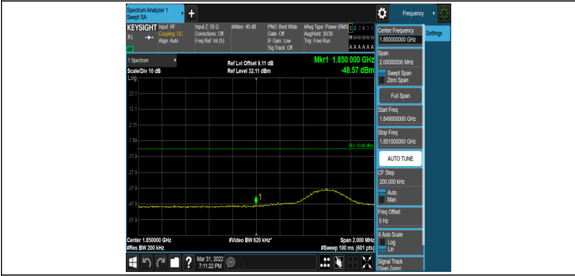
Band2-10MHz-16QAM-18650-1RB#49
