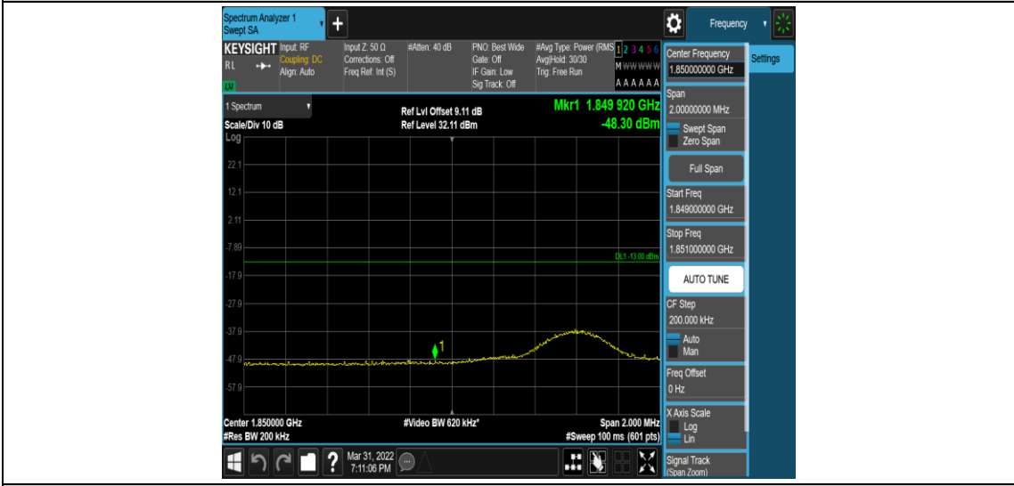
Band2-10MHz-QPSK-18650-1RB#49
