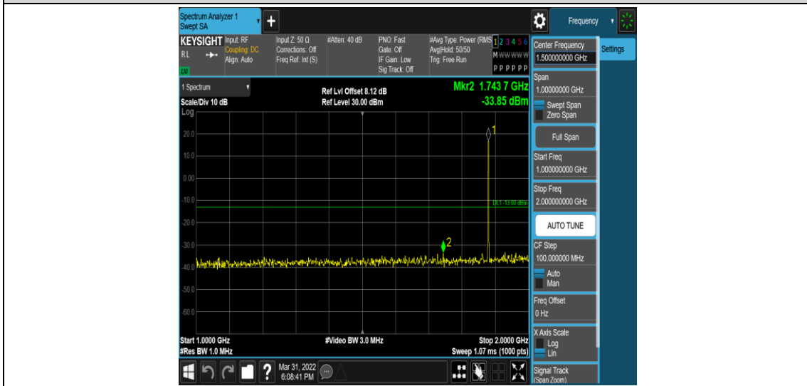
Band2-1.4MHz-QPSK-18900-1RB#0-Range4:1000~2000MHz
