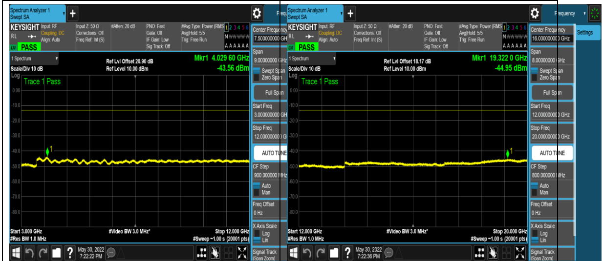
1-N71-PC3-15-15-L-4-DFT-QPSK-Edge_1RB _Left-1 @ 0-3000-12000--43.56--13-PASS
