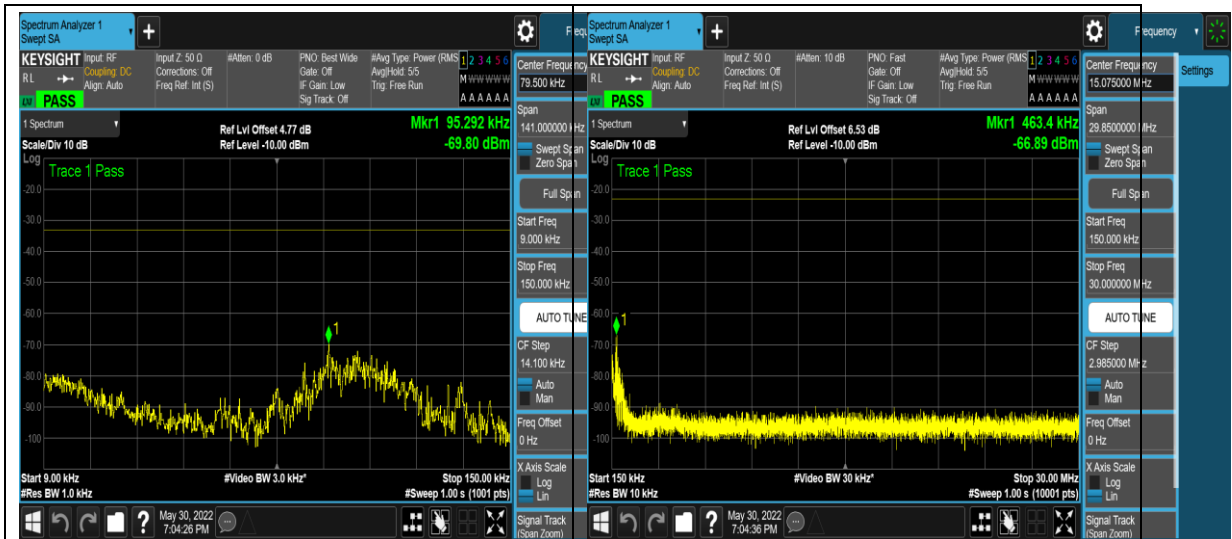
1-N71-PC3-15-10-M-16-CP-QPSK-Edge_1R B_Left-1@0-0.009-0.15--69.80--33-PASS
