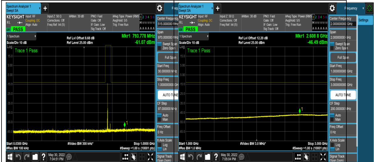
1-N71-PC3-15-10-M-16-CP-QPSK-Edge_1R B_Left-1@0-30-1000--61.07--13-PASS
