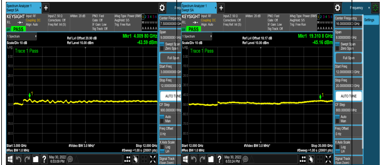
1-N71-PC3-15-10-L-16-CP-QPSK-Edge_1R B_Left-1@0-3000-12000--43.59--13-PASS
