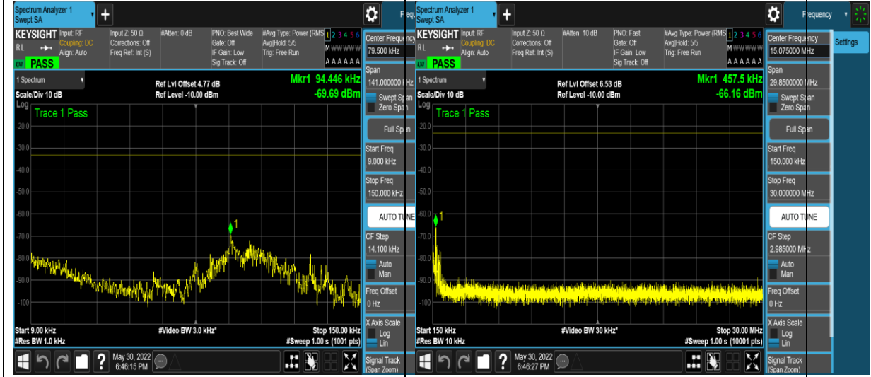
1-N71-PC3-15-10-L-4-DFT-QPSK-Edge_1RB _Left-1@0-0.009-0.15--69.69--33-PASS
