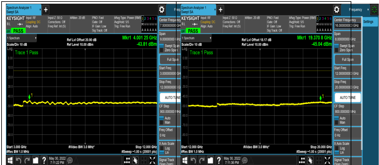
1-N71-PC3-15-10-H-4-DFT-QPSK-Edge_1R B_Left-1@0-3000-12000--43.81--13-PASS
