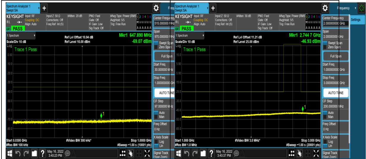
1-N41-PC3-30-80-M-4-DFT-QPSK-Edge_1R B_Left-1@0-30-1000--69.07--35-PASS
