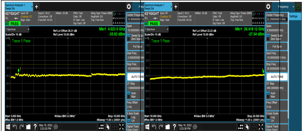
1-N41-PC3-30-60-H-16-CP-QPSK-Edge_1R B_Left-1@0-3000-18000--35.92--25-PASS
