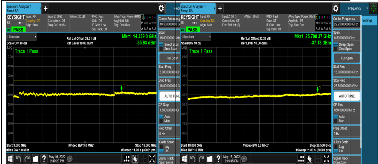
1-N41-PC3-30-60-L-4-DFT-QPSK-Edge_1RB _Left-1 @ 0-3000-18000--35.93--25-PASS
