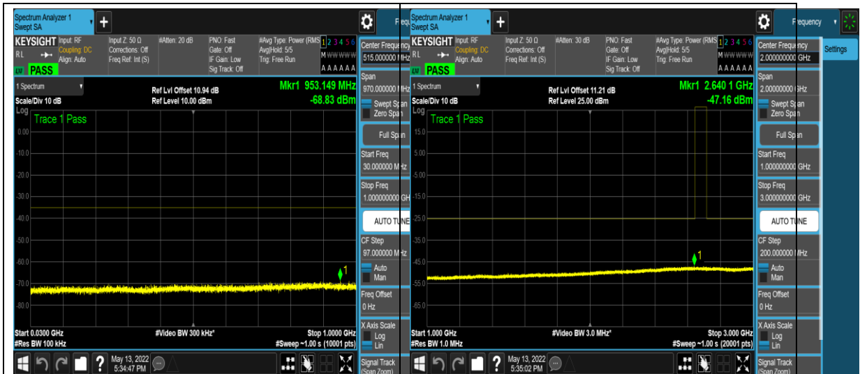
1-N41-PC3-30-20-H-4-DFT-QPSK-Edge_1R B_Left-1@0-30-1000--68.83--35-PASS
