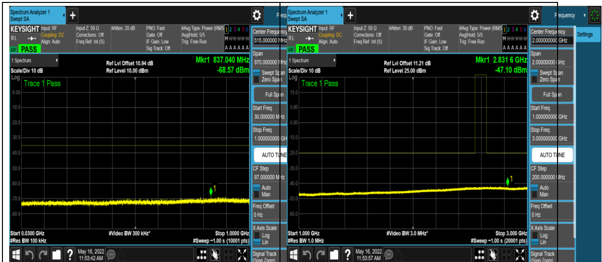
1-N41-PC3-30-30-M-16-CP-QPSK-Edge_1R B_Left-1@0-30-1000--68.57--35-PASS
