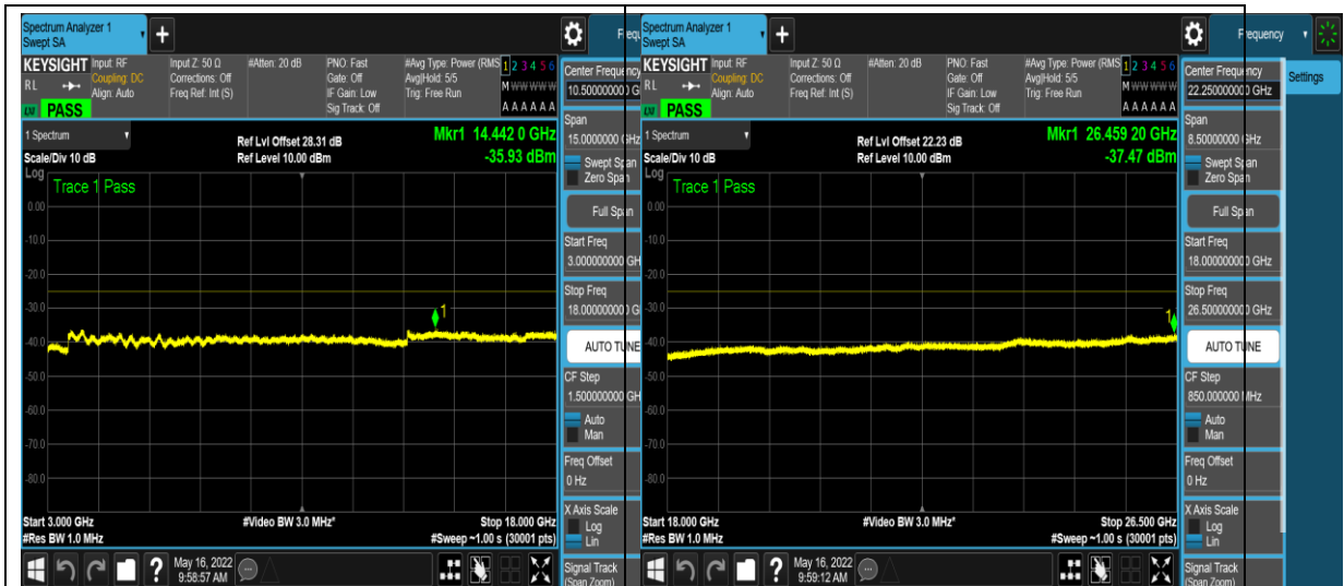
1-N41-PC3-30-30-L-4-DFT-QPSK-Edge_1RB _Left-1@0-3000-18000--35.93--25-PASS
