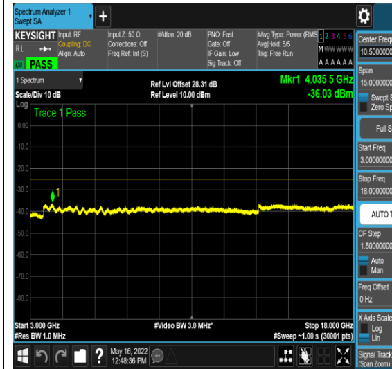
1-N41-PC3-30-40-L-4-DFT-QPSK-Edge_1RB _Left-1@0-30-1000--69.33--35-PASS
