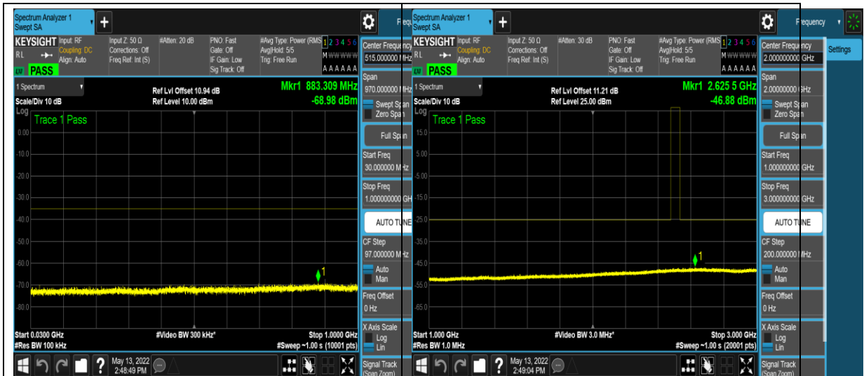
1-N41-PC3-30-15-L-4-DFT-QPSK-Edge_1RB _Left-1 @ 0-30-1000--68.98--35-PASS
