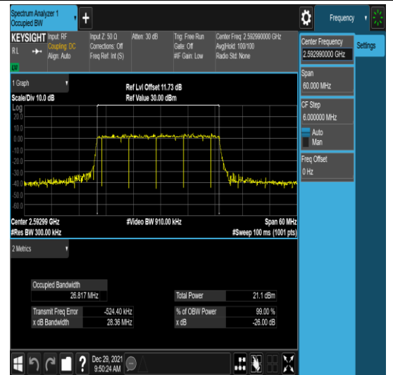
n41-PC3-30-30-M-4-N/A-N/A-N/A-DFT-64QA M-Outer_Full-75@0-Ant1-26.817-28.36≤30- PASS
