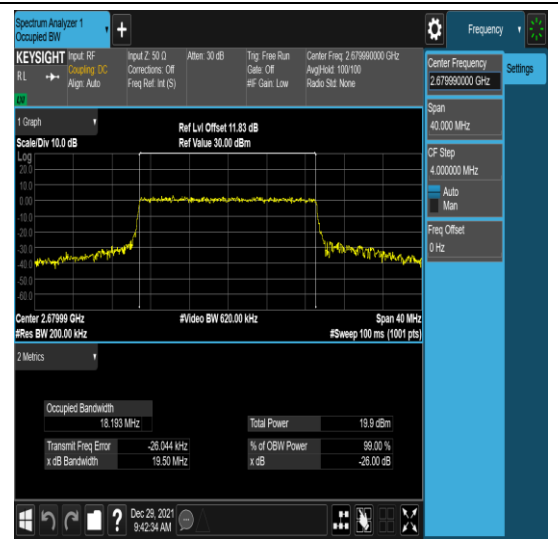
n41-PC3-30-20-H-6-N/A-N/A-N/A-CP-16QAM-Outer_Full-51@0-Ant1-18.193-19.50-≤20-PASS
