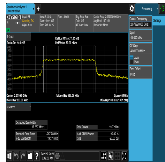
n41-PC3-30-20-H-5-N/A-N/A-N/A-CP-QPSK-Outer_Full-51@0-Ant1-17.857-19.27-≤20-PA SS
