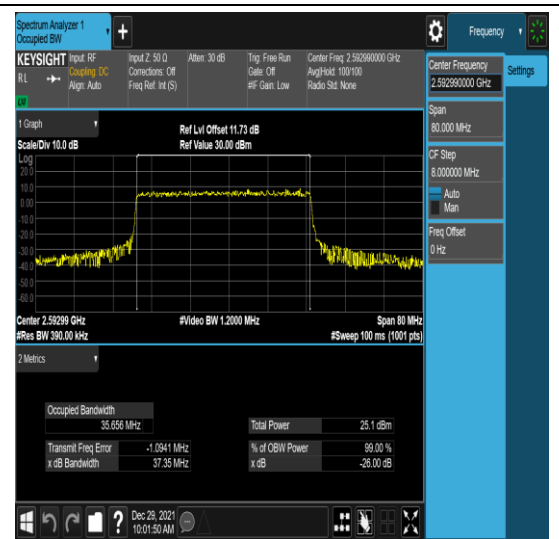
n41-PC3-30-40-M-2-N/A-N/A-N/A-DFT-PI2B PSK-Outer_Full-100@0-Ant1-35.656-37.35-≤40-PASS
