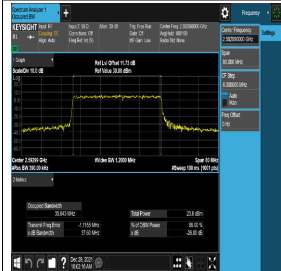
n41-PC3-30-40-M-3-N/A-N/A-N/A-DFT-16QA M-Outer_Full-100@0-Ant1-35.643-37.60-≤40-PASS
