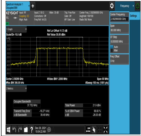
n41-PC3-30-40-M-7-N/A-N/A-N/A-CP-64QAM-Outer_Full-106@0-Ant1-37.752-39.48-<40 -PASS
