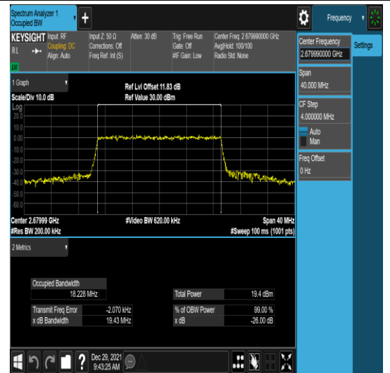
n41-PC3-30-20-H-8-N/A-N/A-N/A-CP-256QAM-Outer_Full-51@0-Ant1-18.228-19.43-≤20-PASS
