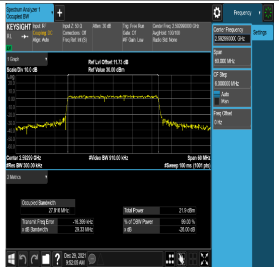
n41-PC3-30-30-M-8-N/A-N/A-N/A-CP-256QA M-Outer_Full-78@0-Ant1-27.816-29.33-≤30- PASS
