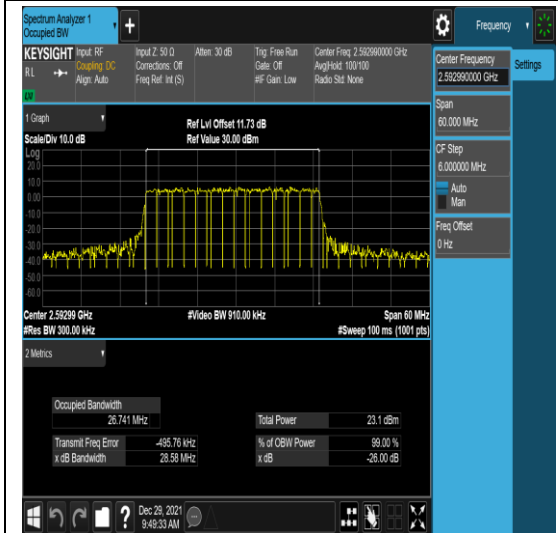
n41-PC3-30-30-M-3-N/A-N/A-N/A-DFT-16QA M-Outer_Full-75@0-Ant1-26.741-28.58≤30- PASS
