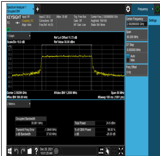
n41-PC3-30-40-M-1-N/A-N/A-N/A-DFT-QPS K-Outer_Full-100@0-Ant1-35.661-37.63-≤40-PASS
