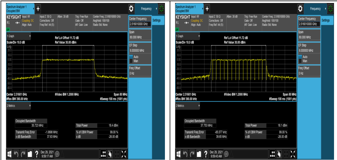
n41-PC3-30-40-L-5-N/A-N/A-N/A-CP-QPSK- Outer_Full-106@0-Ant1-35.723-37.63-≤40-P ASS
