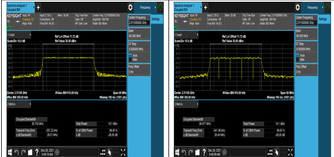
n41-PC3-30-30-L-3-N/A-N/A-N/A-DFT-16QA M-Outer_Full-75@0-Ant1-26.753-28.51-≤30- PASS
