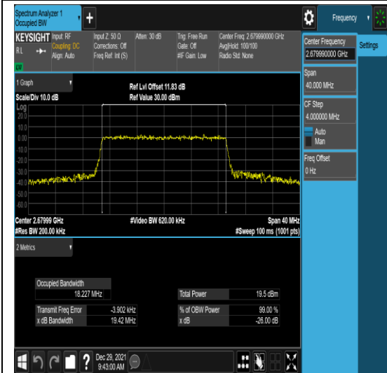
n41-PC3-30-20-H-7-N/A-N/A-N/A-CP-64QAM-Outer_Full-51@0-Ant1-18.227-19.42-≤20-PASS
