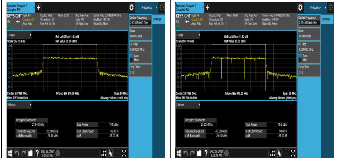
n41-PC3-30-30-H-7-N/A-N/A-N/A-CP-64QAM-Outer_Full-78@0-Ant1-27.840-29.31-≤30-PASS
