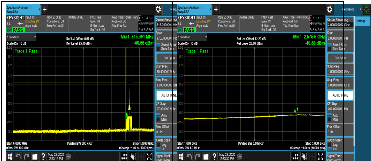
1-N5-PC3-15-10-M-4-DFT-QPSK-Edge_1RB _Left-1 @ 0-30-1000--50.55--13-PASS
