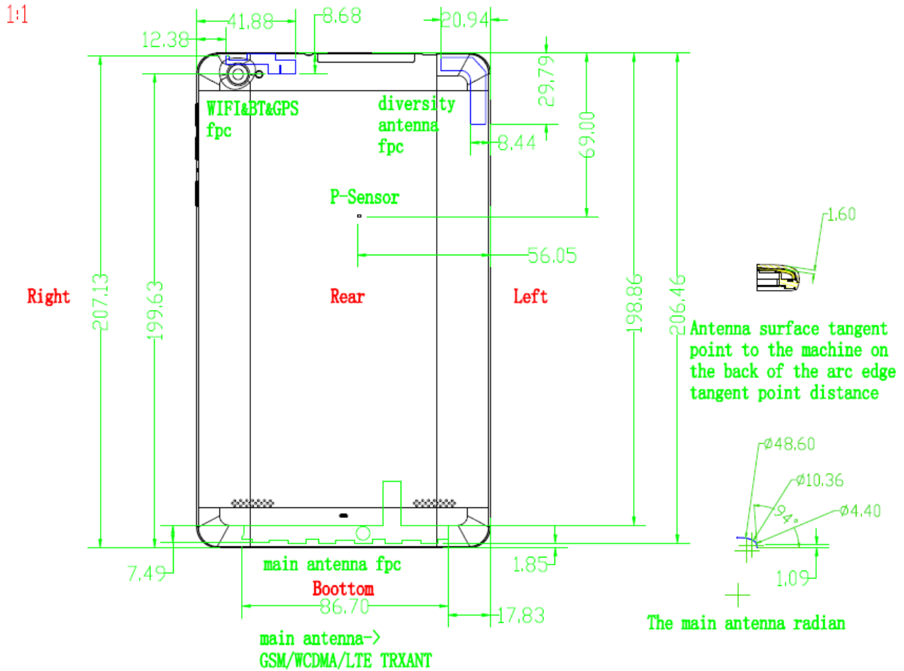
Fig.11.1 EUT Antenna Locations
