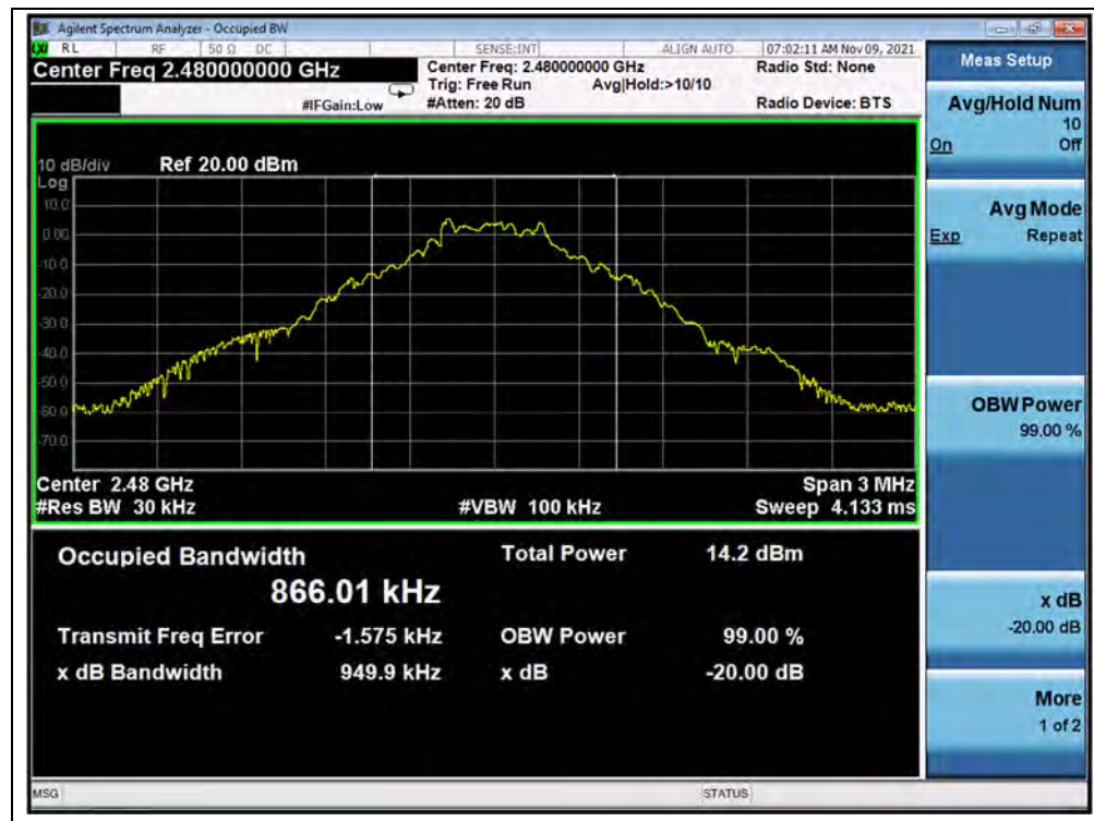
(Channel 78, GFSK)
