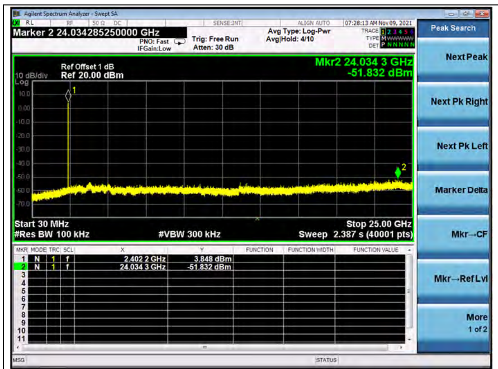
(30MHz to 25GHz, Channel 0, 8-DPSK)
