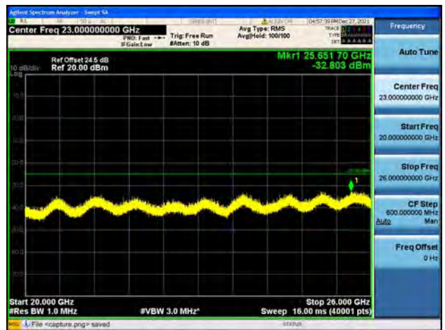
Band7-20G-26G / 10MHz / High CH / 64QAM
