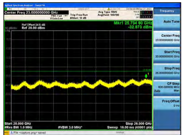
Band7-20G-26G / 15MHz / Low CH / 16QAM
