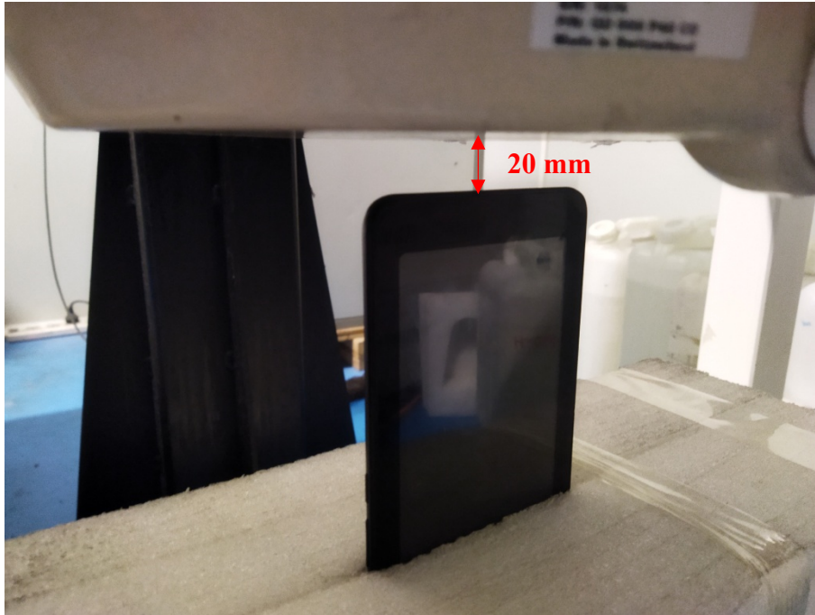
Body Bottom Setup Photo (20mm)
