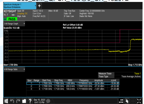
B66_20M_QPSK_100@0_CH_132072
