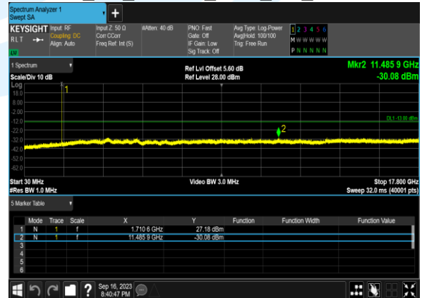
B66_3M_16QAM_1@0_CH_131987
