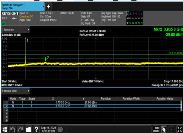
B66_10M_QPSK_1@0_CH_132622
