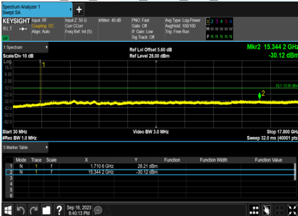
B66_3M_QPSK_1@0_CH_131987
