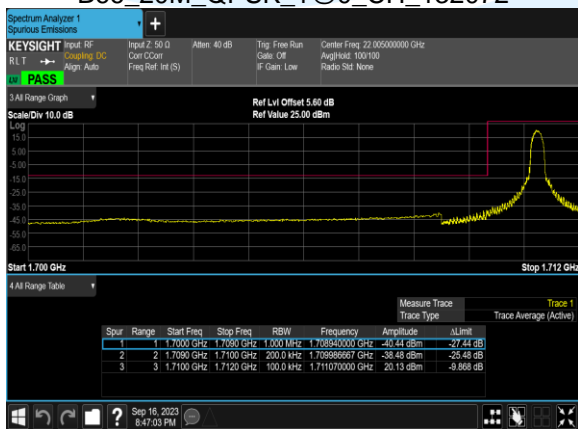
B66_20M_QPSK_1@0_CH_132072
