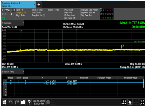
B66_20M_QPSK_1@0_CH_132072
