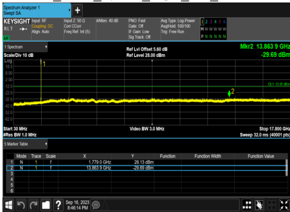
B66_1.4M_QPSK_1@0_CH_132665
