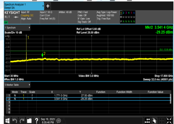
B66_10M_16QAM_1@0_CH_132622
