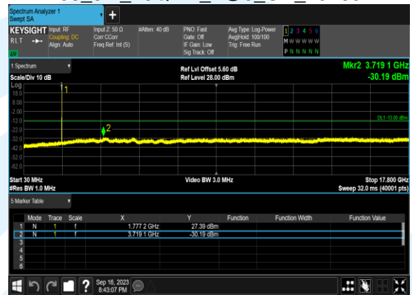
B66_1.4M_16QAM_1@0_CH_131979
