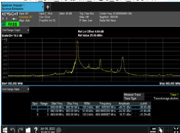
B71_5M_16QAM_1@0_CH_133147
