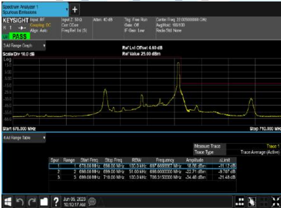
B71_5M_16QAM_1@24_CH_133447
