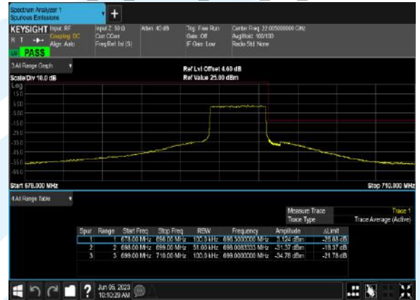
B71_5M_16QAM_25@0_CH_133447
