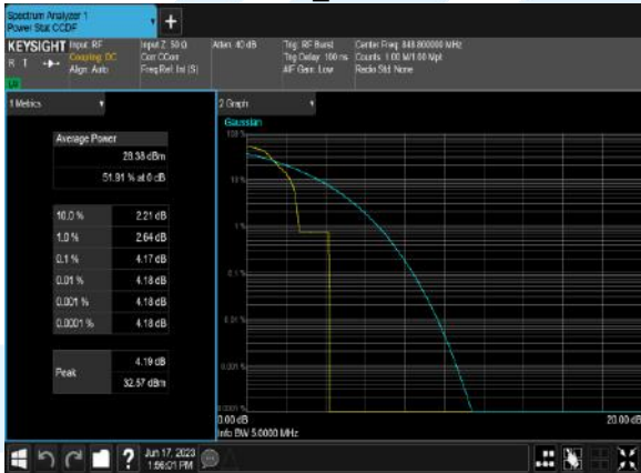
EGPRS850_Channel251
