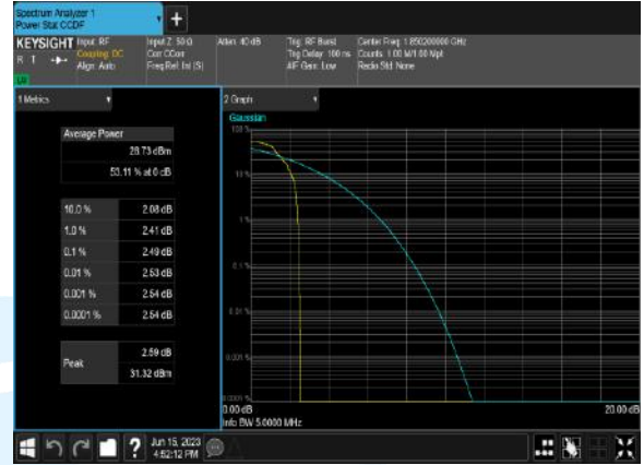
EGPRS1900_Channel512
