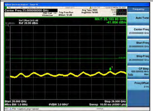
Band7-20G-26G / 15MHz / High CH / 64QAM
