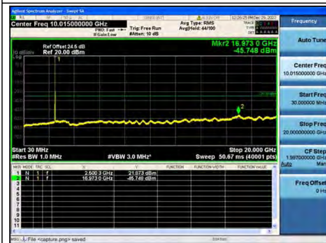
Band7-30M-20G / 15MHz / Low CH / 64QAM
