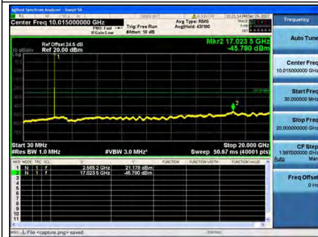
Band7-30M-20G / 5MHz / High CH / 64QAM
