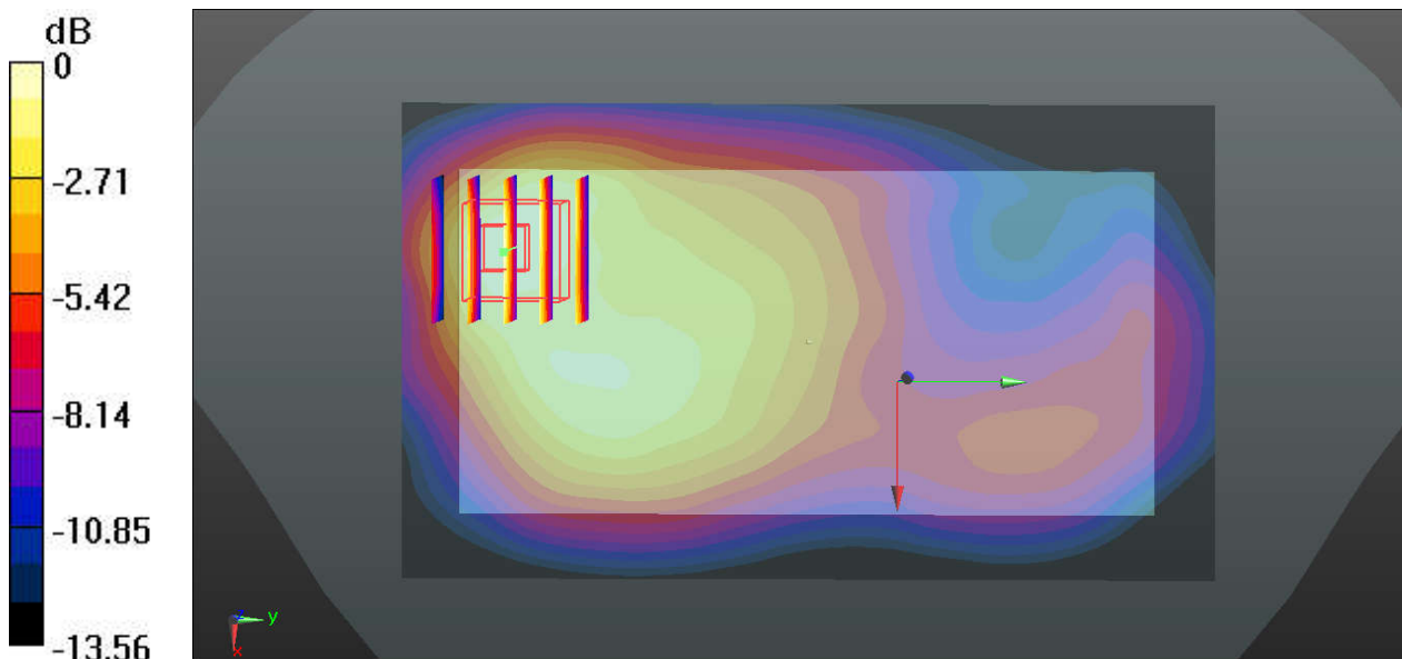
0 dB = 0.913 W/kg
