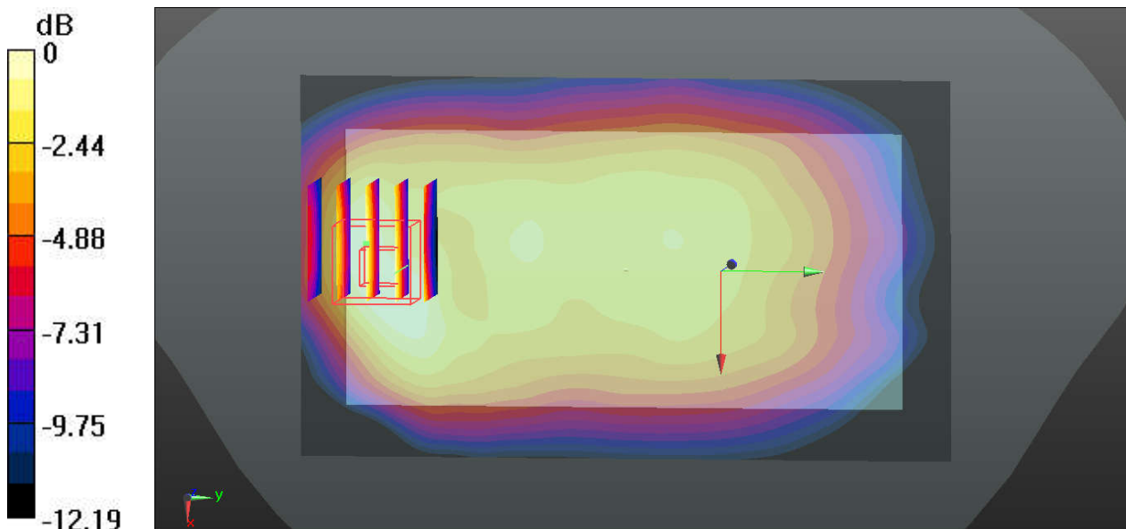
0 dB = 0.299 W/kg
