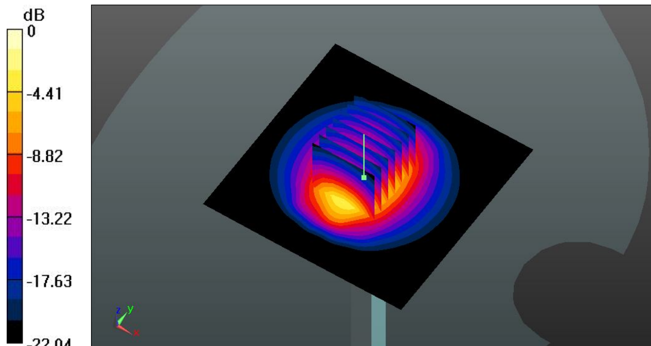
0 dB = 21.5 W/kg
