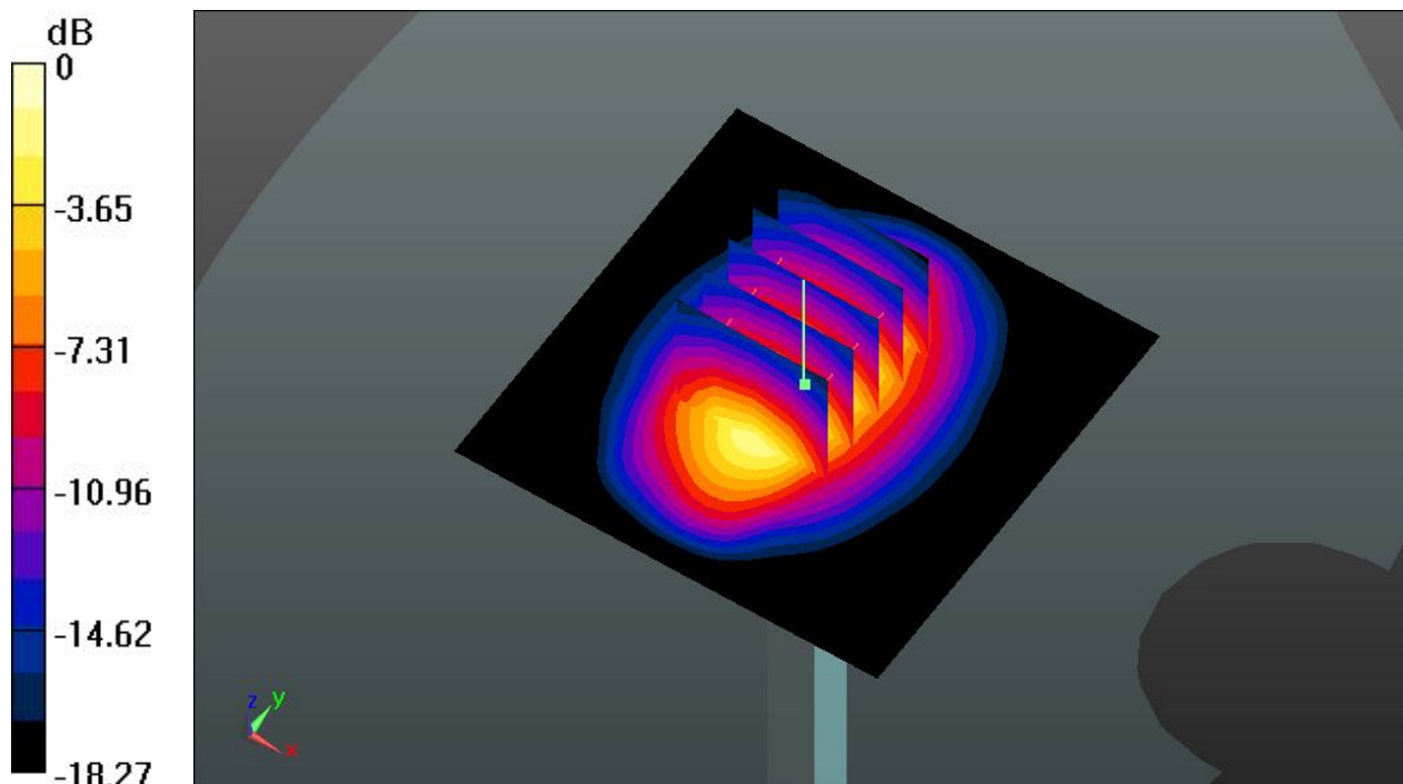
0 dB = 14.8 W/kg
