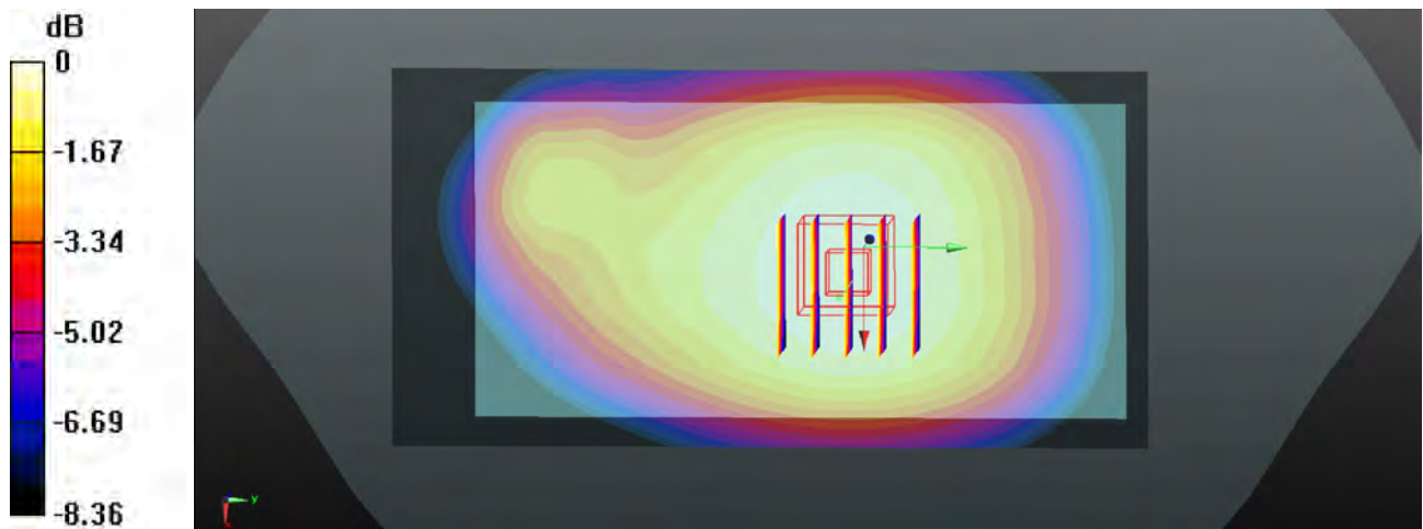
0 dB = 1.02 W/kg
