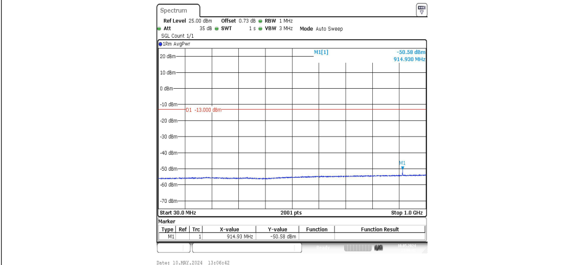
Band2-9262-30~1000MHz-PASS
