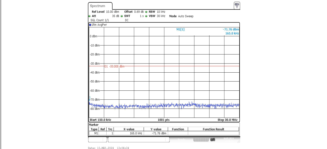
Band2-9262-0.15~30MHz-PASS
