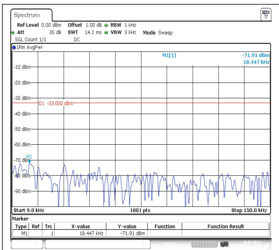
Band71_10MHz_QPSK_133422_1RB#0_0.009~0.15_0.009~0.15
