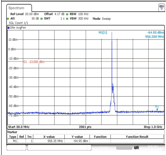
Band71_10MHz_QPSK_133297_1RB#0_30~100_0_30~1000
