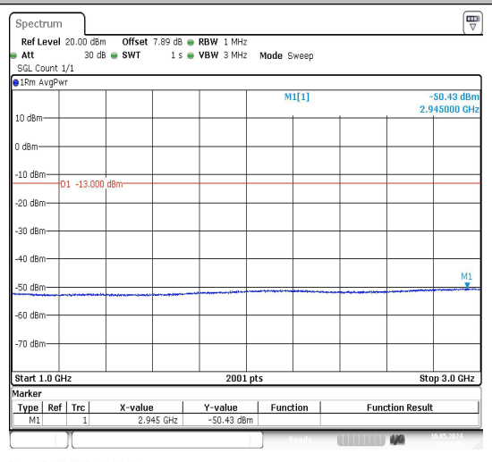
Band71_10MHz_QPSK_133422_1RB#0_1000~3000_00_1000~3000
