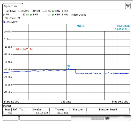
Band71_5MHz_16QAM_133147_1RB#0_3000~10000 000_3000~10000
