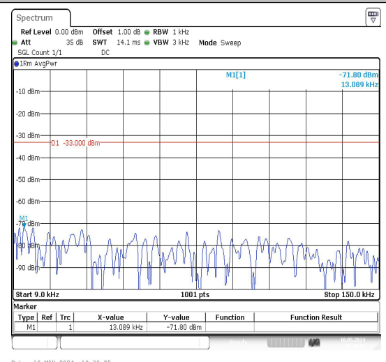
Band71_10MHz_QPSK_133297_1RB#0_1000~3000_00_1000~3000
