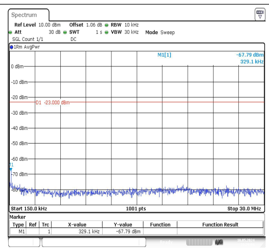
Band71_10MHz_QPSK_133297_1RB#0_0.15~30_0.15~30
