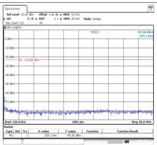
Band71_10MHz_QPSK_133422_1RB#0_0.15~30_0.15~30
