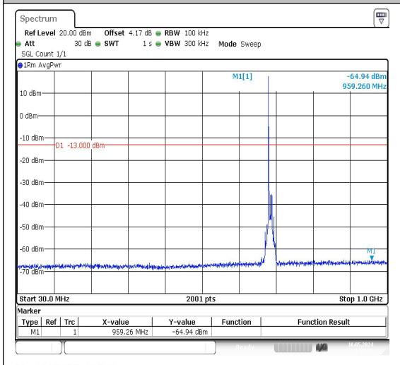
Band71_10MHz_QPSK_133422_1RB#0_30~100_0_30~1000
