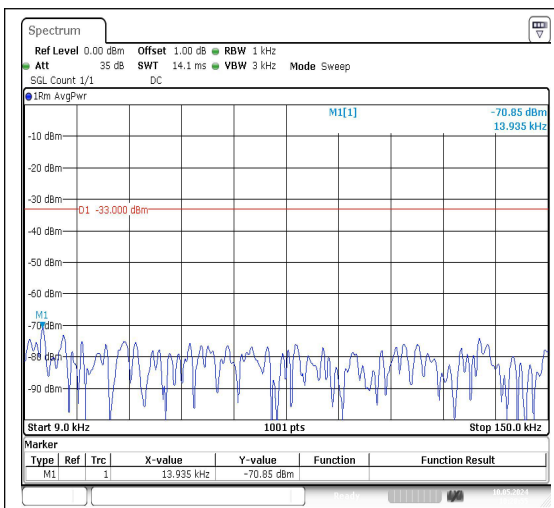
Band71_10MHz_QPSK_133297_1RB#0_0.009~0.15_0.009~0.15
