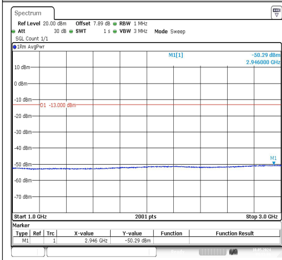
Band71_5MHz_16QAM_133147_1RB#0_1000~3000 000_1000~3000
