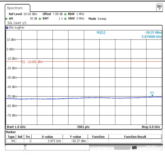
Band71_10MHz_QPSK_133297_1RB#0_1000~3000_00_1000~3000
