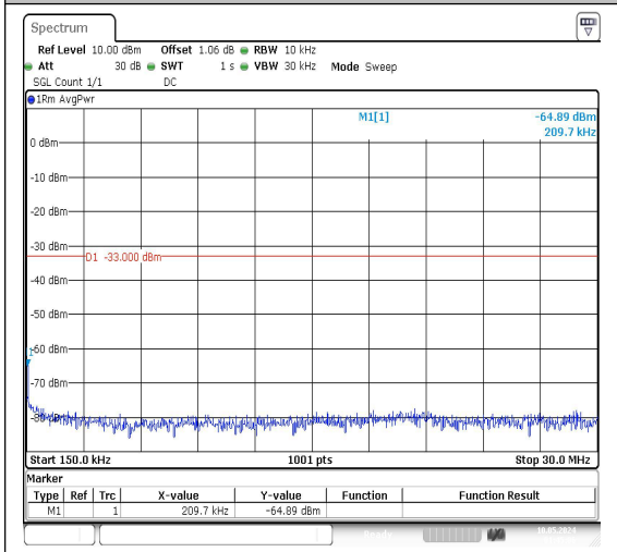
Band66_10MHz_QPSK_132022_1RB#0_3000~20000 0000_3000~20000
