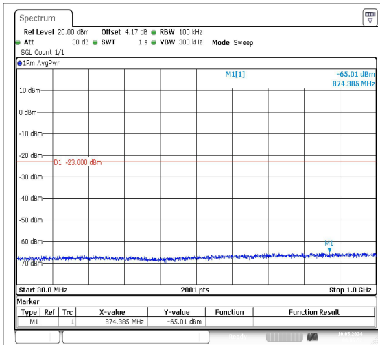
Band66_1.4MHz_QPSK_132322_1RB#0_30~100 0_30~1000
