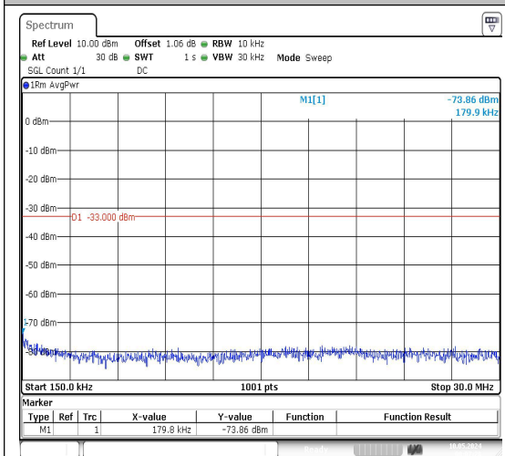
Band66_1.4MHz_QPSK_132322_1RB#0_3000~2 0000_3000~20000
