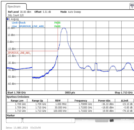
Band66_3MHz_QPSK_131987_1RB#0
