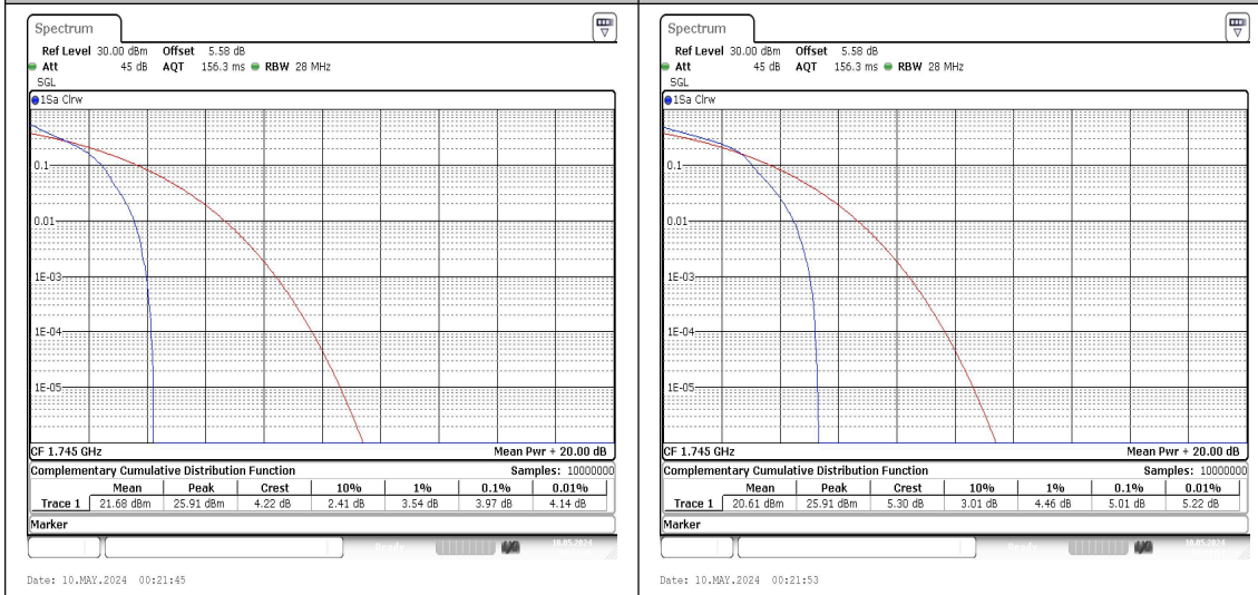
Band66-1.4MHz-QPSK-132322-1RB#0-PASS Band66-1.4MHz-16QAM-132322-1RB#0-PASS
